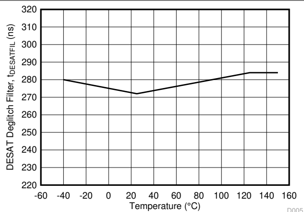
6-28. t_{\text{DESATFIL}} DESAT Deglitch Filter vs Temperature
