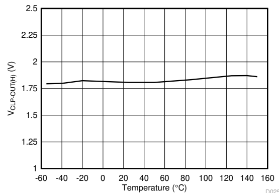
FIG 6-19. V_{CLP-OUT(H)} Short Circuit Clamping Voltage vs Temperature
