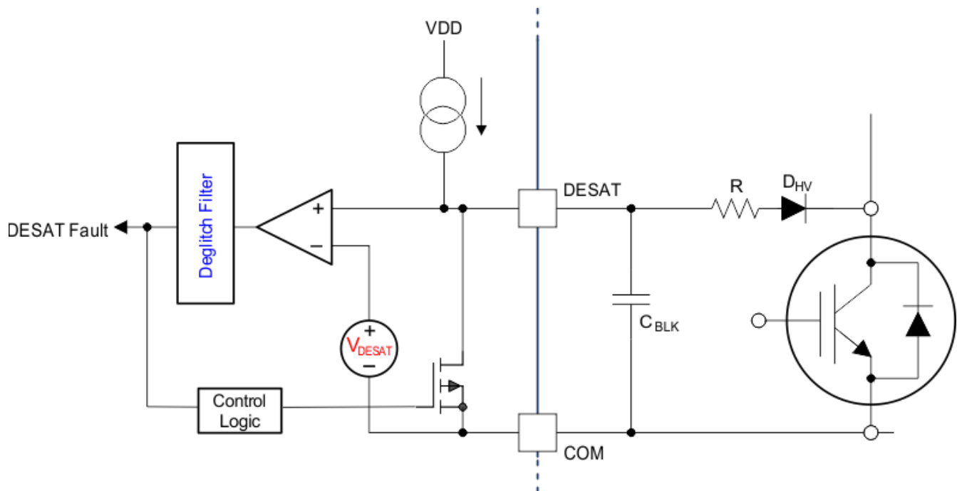
FIG 8-5. DESAT Protection
