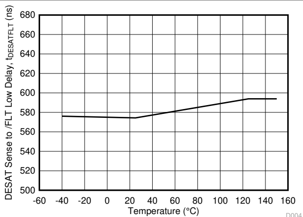
FIG 6-27. t_{DESATFLT} DESAT Sense to /FLT Low Delay Time vs Temperature
