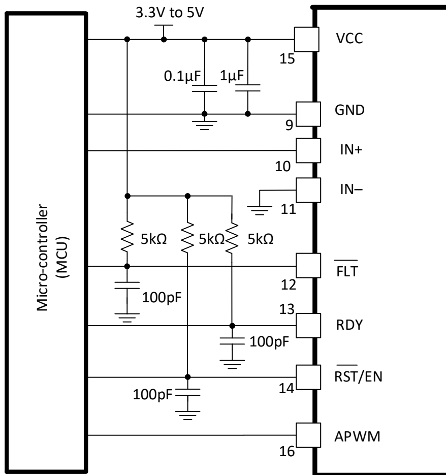
FIGURE 9-3. \overline{\text{FLT}} , \text{RDY} , and \overline{\text{RST/EN}} Pins Circuitry
