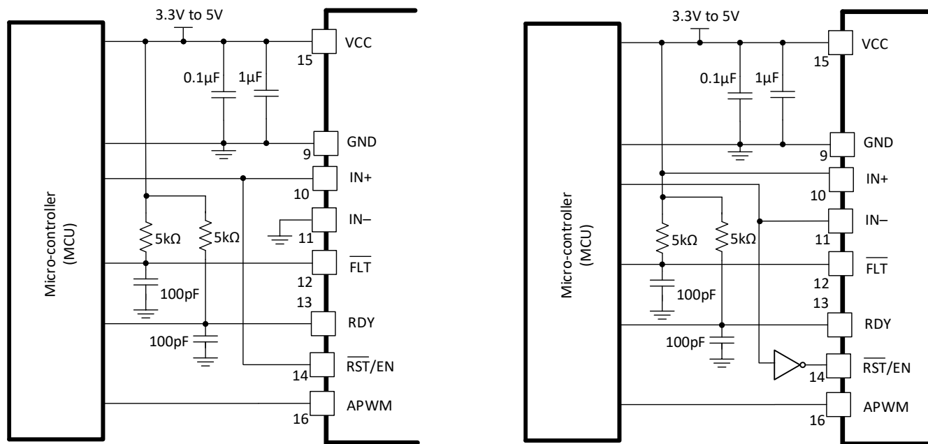
FIG 9-4. Automatic Reset Control
