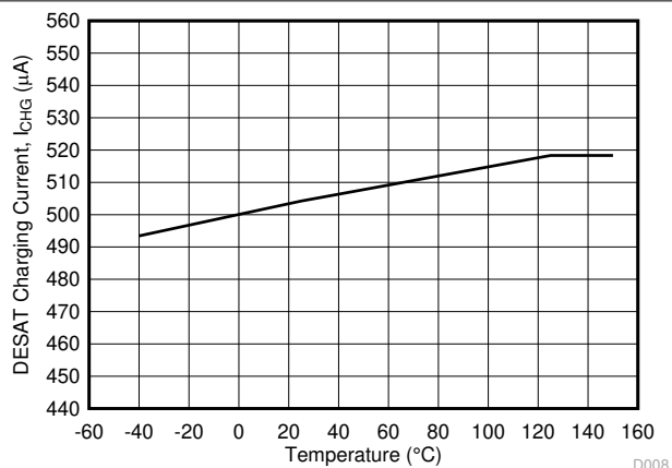
6-29. I_{\text{CHG}} DESAT Charging Current vs Temperature
