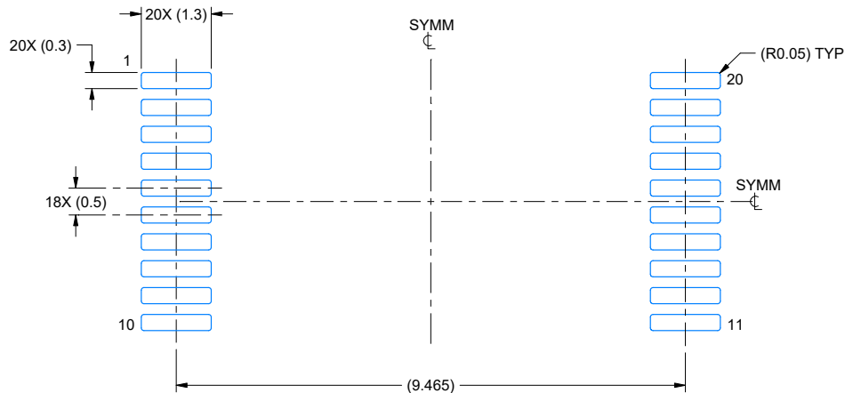
LAND PATTERN EXAMPLE EXPOSED METAL SHOWN SCALE: 10X
