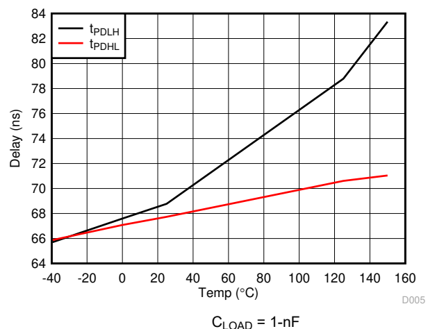
Figure 6-8. Propagation delay versus Temperature
