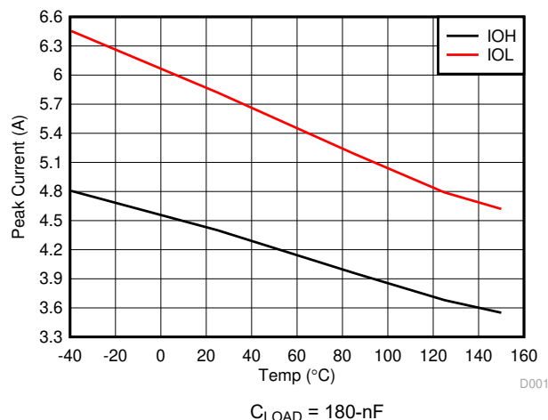
Figure 6-4. Output Drive currents versus Temperature
