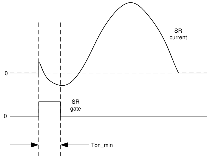
FIG 8-8. SR current with leading edge spike
