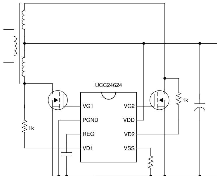
FIG 8-9. UCC24624 configuration with VD resistors
