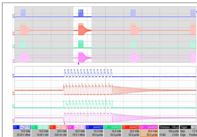
FIG 9-6. V_{IN} = 390\text{ V} , I_{OUT} = 0.3\text{ A} , LLC is Operating In Burst Mode
