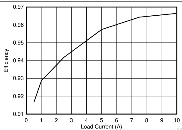
FIG 9-11. V_{IN} = 390\text{ V} , Power Converter System Efficiency Using SR FETs
