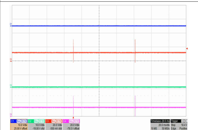
9-5. V_{IN} = 390 V, I_{OUT} = 0 A, No Gate Drive Under Light Load (VG1, VG2)
