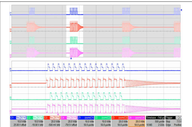
9-3. V_{IN} = 340 V, I_{OUT} = 0.3 A, LLC is Operating In Burst Mode
