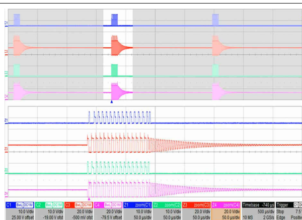
FIG 9-9. V_{IN} = 410\text{ V} , I_{OUT} = 0.3\text{ A} , LLC is Operating In Burst Mode
