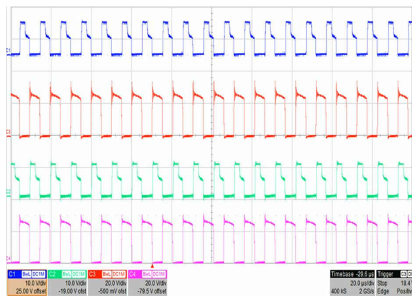
FIG 9-7. V_{IN} = 390\text{ V} , I_{OUT} = 10\text{ A} Full Load
