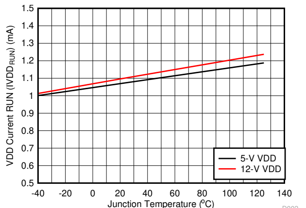
7-2. Bias Supply Current vs Temperature (No Switching)
