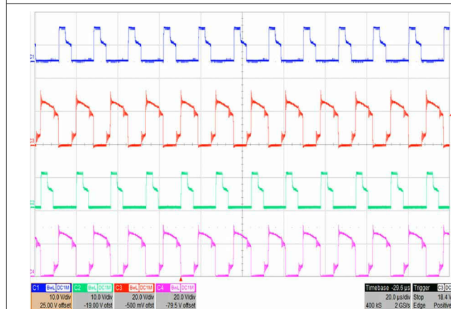
9-4. V_{IN} = 340 V, I_{OUT} = 10 A Full Load
