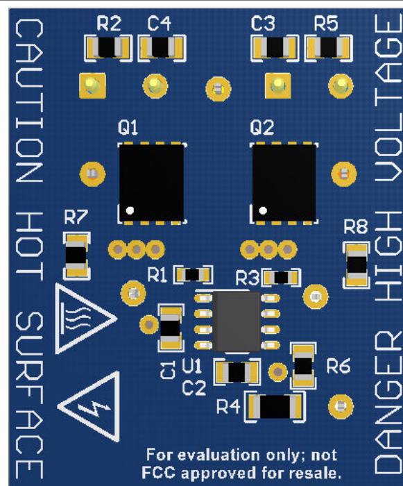
11-3. UCC24624EVM-015 (Bottom View)
