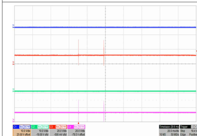
FIG 9-8. V_{IN} = 410\text{ V} , I_{OUT} = 0\text{ A} , No Gate Drive Under Light Load (VG1, VG2)
