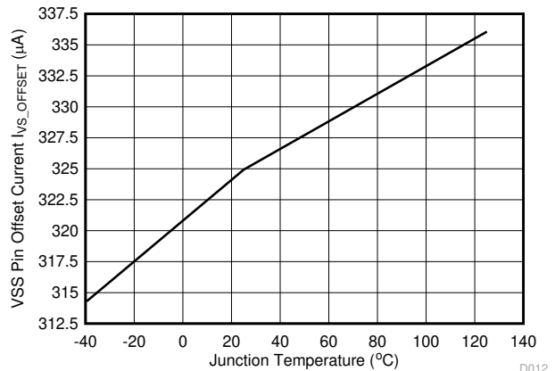
7-12. VSS Pin Offset Current vs Temperature
