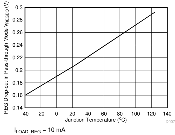
7-7. REG Dropout in Pass-through Mode vs Temperature
