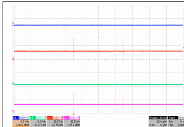
9-2. V_{IN} = 340 V, I_{OUT} = 0 A, No Gate Drive Under Light Load (VG1, VG2)
