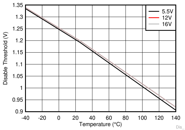
6-11. Disable Threshold
