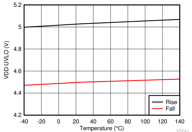
6-14. VDD UVLO Threshold
