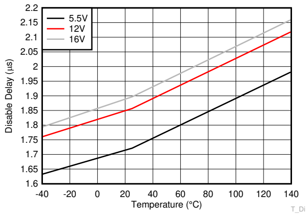
6-13. Disable Delay
