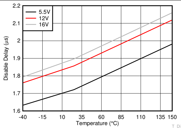
FIG 6-13. Disable Delay
