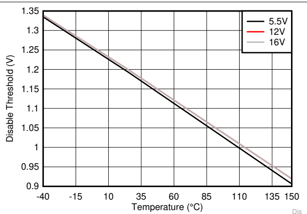
FIG 6-11. Disable Threshold
