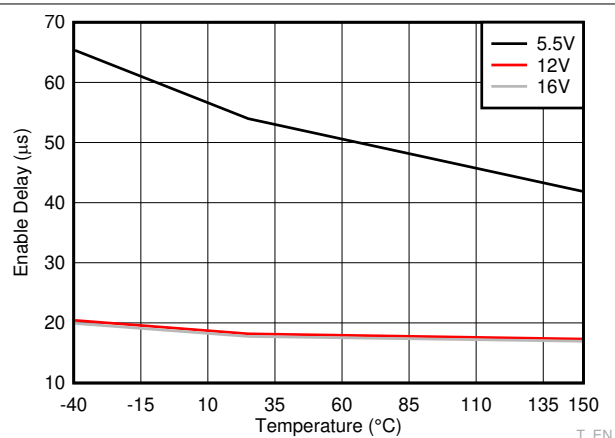
FIG 6-12. Enable Delay
