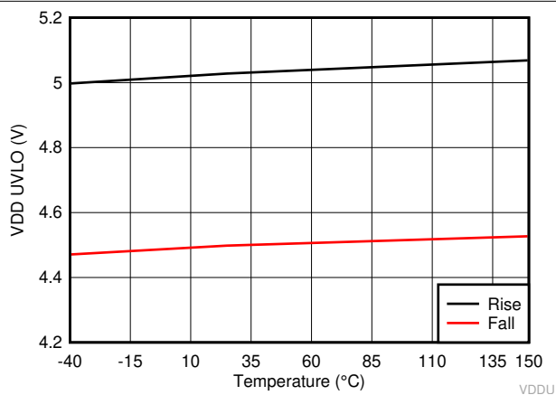
FIG 6-14. VDD UVLO Threshold
