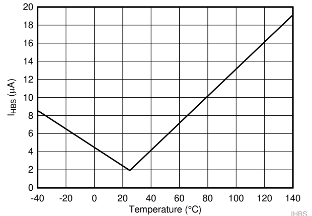
A. V_{HB} = V_{HS} = 100\text{ V} 图 6-6. HB to VSS Quiescent Current
