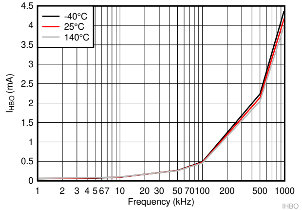
A. C_L = 0\text{ F} V_{DD} = V_{HB} = 12\text{ V} 图 6-4. HB Operating Current
