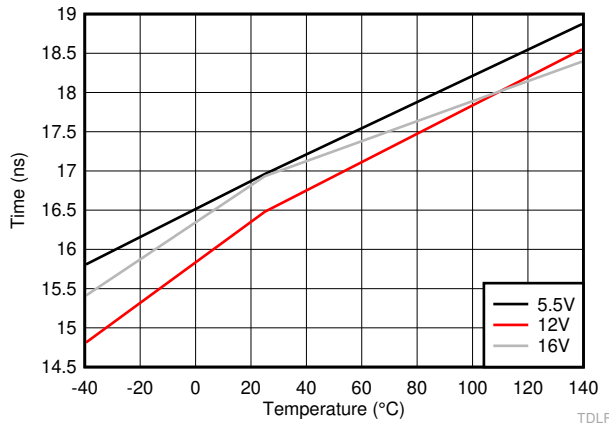
C_L=No\ Load 6-31. LO Falling Propagation Delay (TDLFF)
