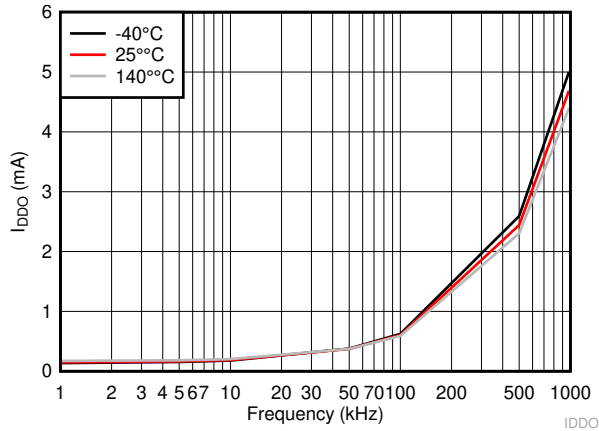
A. C_L = 0\text{ F} V_{DD} = V_{HB} = 12\text{ V} 图 6-3. VDD Operating Current
