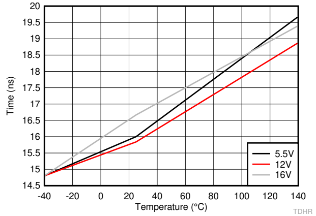
C_L=No\ Load 6-28. HO Rising Propagation Delay (TDHR)
