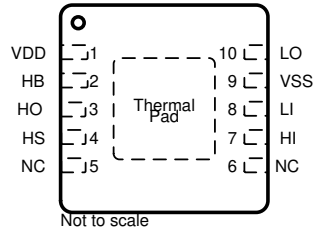
5-3. DPR Package 10-Pin SON Top View
