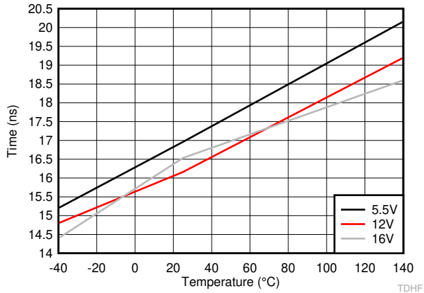
C_L=100nF 6-27. HO Rise andamp; Fall Time
