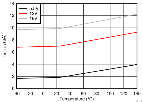
A. C_L = 0\text{ F} V_{EN} = 0\text{ V} 图 6-5. VDD Current When Disabled
