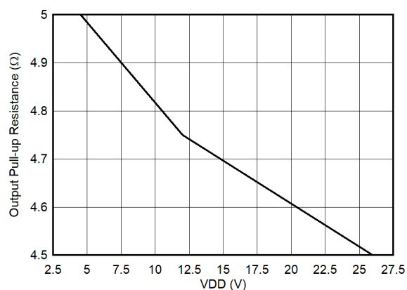
Figure 6-12. Output Pullup Resistance
