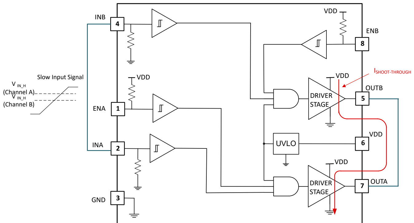
図 6-2. Slow Input Signal Can Cause Shoot-Through Between Channels During Paralleling (Recommended DV/DT is 20 V/Ms or Higher)
