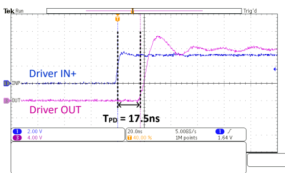
FIG 8-3. UCC27614 Rising (Turn-On) Propagation Delay
