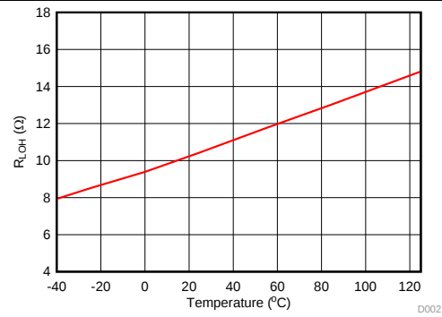
21. LO Output Pull-Up Resistance vs Temperature
