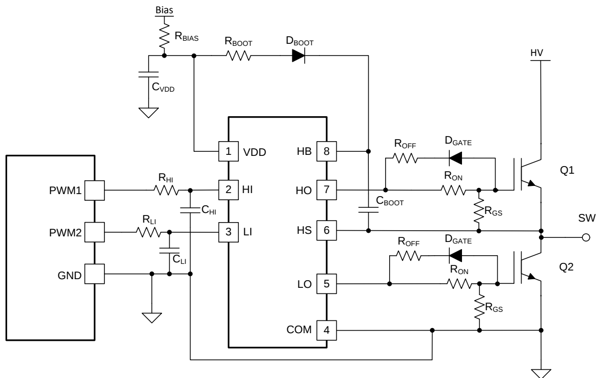
46. Typical IGBT Application Schematic
