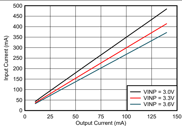
図 6-17. Input Current ( I_{VINP} ) vs Load Current ( I_{VCC} ): V_{CC} = 5.0V , T_A = 25^\circ C , C_{OUT2} = 22\mu F
