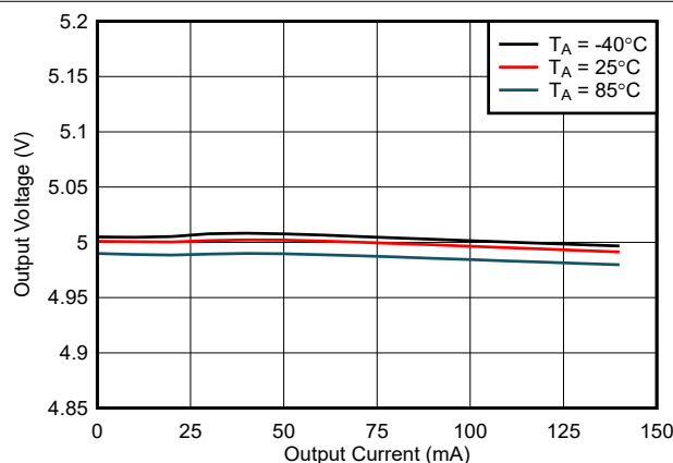
6-23. Output Voltage Regulation ( V_{VCC} ) vs Load Current ( I_{VCC} ): V_{CC} = 5.0V , V_{INP} = 3.3V , C_{OUT2} = 22\mu F
