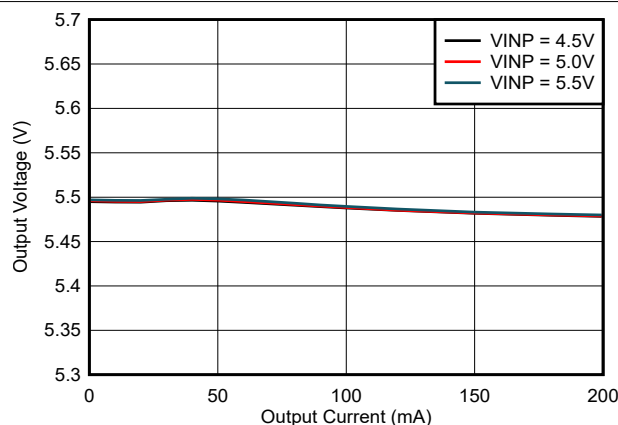
6-21. Output Voltage Regulation ( V_{VCC} ) vs Load Current ( I_{VCC} ): V_{CC} = 5.5V , T_A = 25^\circ C , C_{OUT2} = 22\mu F
