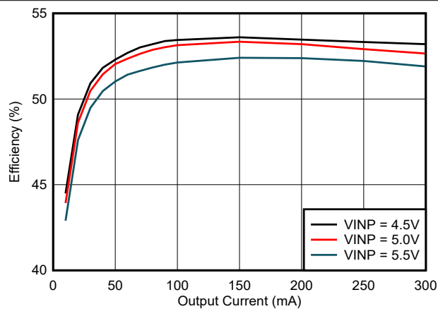
Figure 6-9. Efficiency vs Load Current ( I_{VCC} ): V_{CC} = 5.0V , T_A = 25^\circ C , C_{OUT2} = 22\mu F
