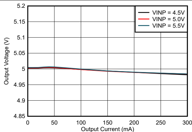
6-19. Output Voltage Regulation ( V_{VCC} ) vs Load Current ( I_{VCC} ): V_{CC} = 5.0V , T_A = 25^\circ C , C_{OUT2} = 22\mu F
