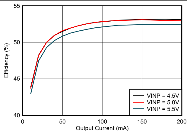
Figure 6-11. Efficiency vs Load Current ( I_{VCC} ): V_{CC} = 5.5V , T_A = 25^\circ C , C_{OUT2} = 22\mu F
