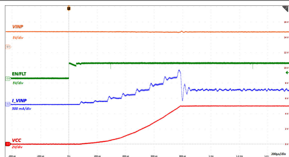
図 6-25. Start-Up with En/FLT From Low to High: VINP = 5.0V , VCC = 5.0V , 18Ω Load
