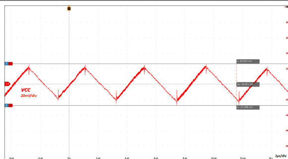
図 6-26. Steady State Output Voltage Ripple: VINP = 5.0V, VCC = 5.0V , C OUT2 = 22μF, 300mA Load
