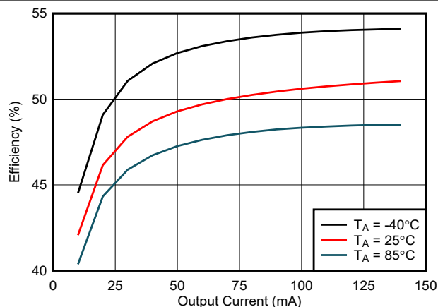
図 6-13. Efficiency vs Load Current ( I_{VCC} ): V_{CC} = 5.0V , V_{INP} = 3.3V , C_{OUT2} = 22\mu F
