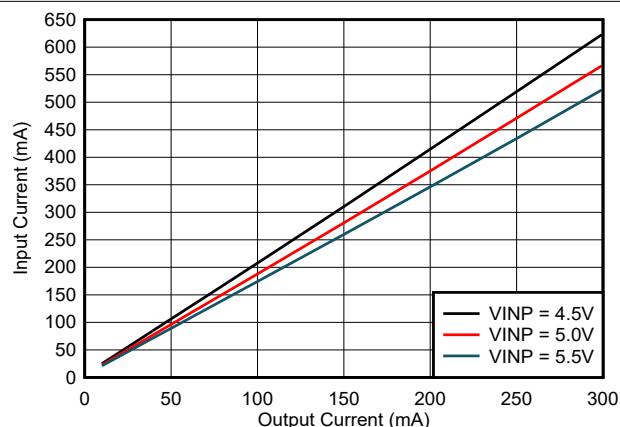
図 6-15. Input Current ( I_{VINP} ) vs Load Current ( I_{VCC} ): V_{CC} = 5.0V , T_A = 25^\circ C , C_{OUT2} = 22\mu F
