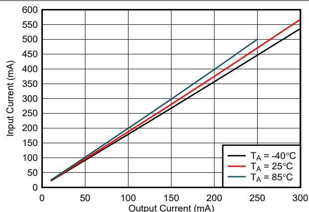
図 6-16. Input Current ( I_{VINP} ) vs Load Current ( I_{VCC} ): V_{CC} = 5.0V , V_{INP} = 5.0V , C_{OUT2} = 22\mu F
