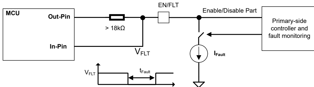
7-6. Fault Reporting Mechanism
