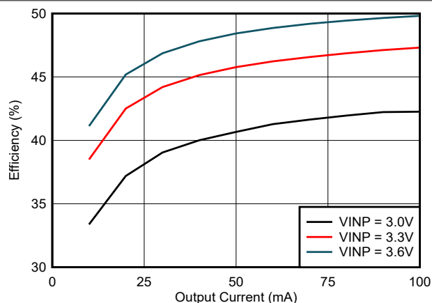
図 6-14. Efficiency vs Load Current ( I_{VCC} ): V_{CC} = 5.5V , T_A = 25^\circ C , C_{OUT2} = 22\mu F
