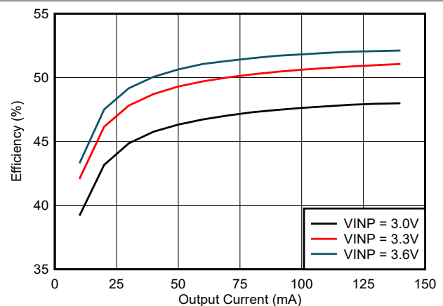
Figure 6-12. Efficiency vs Load Current ( I_{VCC} ): V_{CC} = 5.0V , T_A = 25^\circ C , C_{OUT2} = 22\mu F
