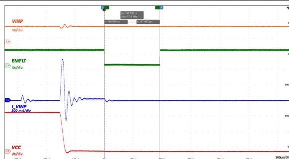
図 6-28. Output Short Circuit Operation: VINP = 5.0V
