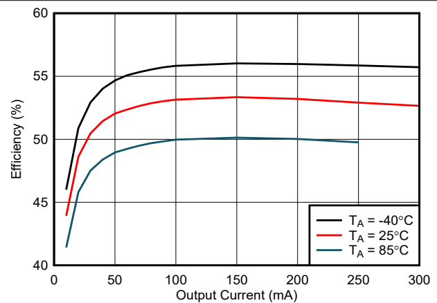
Figure 6-10. Efficiency vs Load Current ( I_{VCC} ): V_{CC} = 5.0V , V_{INP} = 5.0V , C_{OUT2} = 22\mu F
