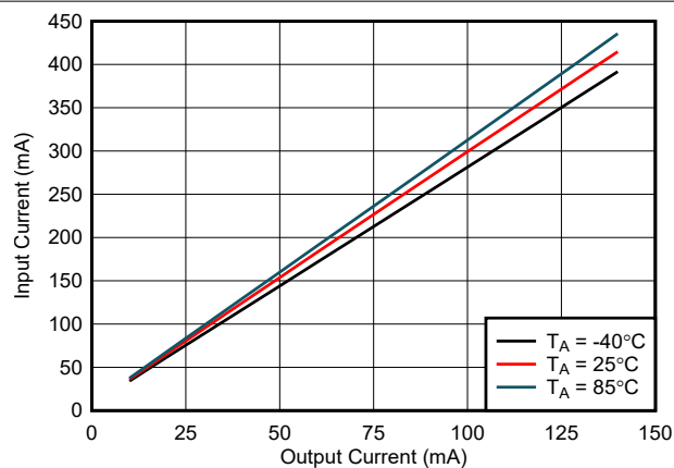
図 6-18. Input Current ( I_{VINP} ) vs Load Current ( I_{VCC} ): V_{CC} = 5.0V , V_{INP} = 3.3V , C_{OUT2} = 22\mu F
