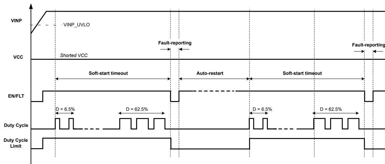
図 7-2. Soft-start under short-circuit output
