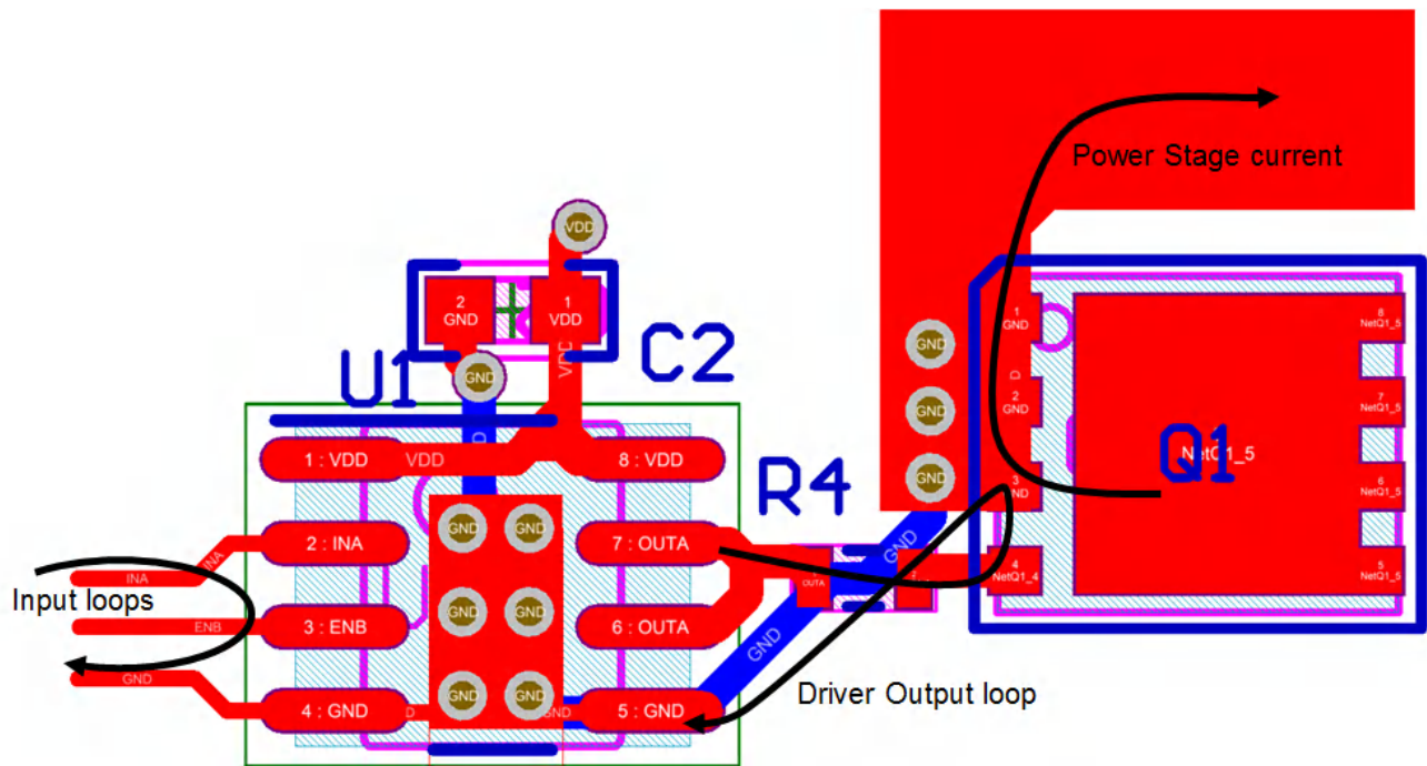
11-1. Layout Recommendation
