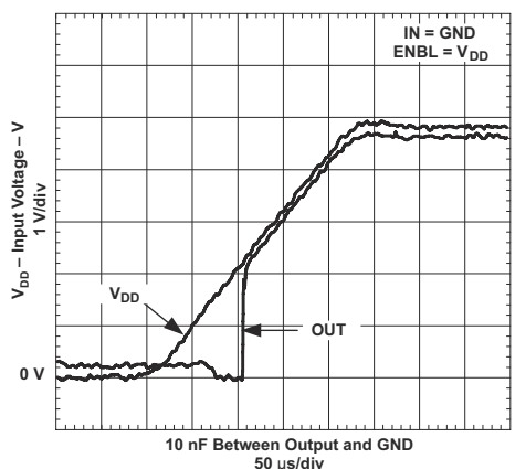
図 7-19. Output Behavior vs V_{DD} (UCC37321)
