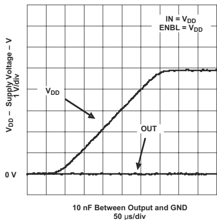
図 7-21. Output Behavior vs VDD (Inverting)
