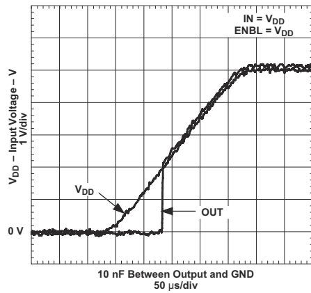
図 9-2. Output Behavior vs VDD (UCC37322)
