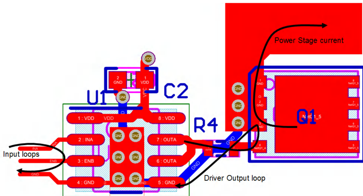
11-1. Layout Recommendation
