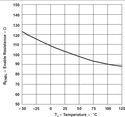
図 7-18. Enable Resistance vs Temperature
