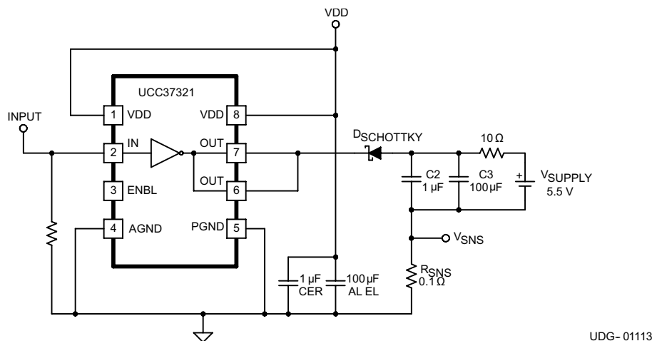
図 8-1. Sink Current Test Circuit
