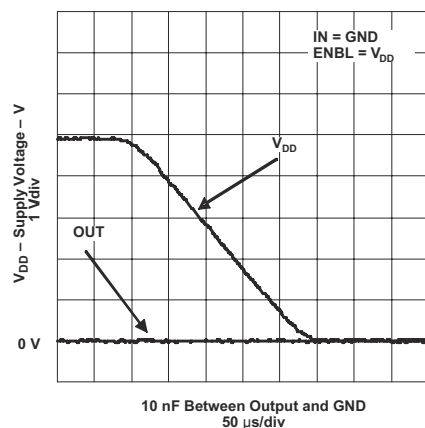
図 7-24. Output Behavior vs VDD (Noninverting)
