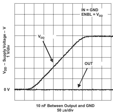
図 7-23. Output Behavior vs VDD (Noninverting)
