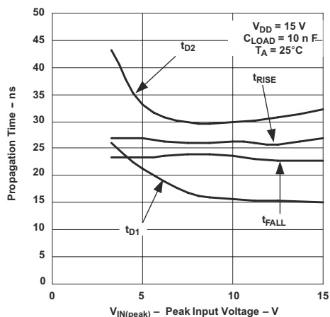
図 7-15. Propagation Times vs Peak Input Voltage
