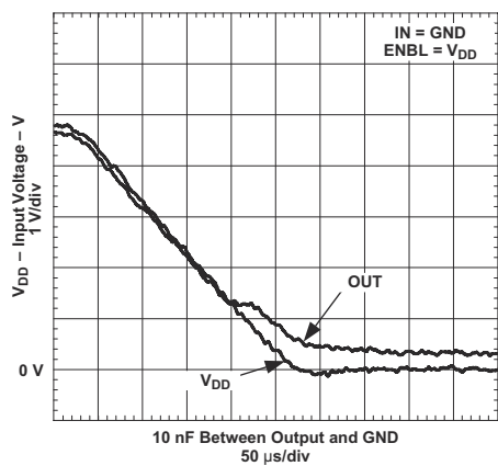
図 7-20. Output Behavior vs V_{DD} (UCC37321)
