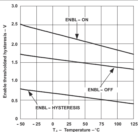
図 7-17. Enable Threshold and Hysteresis vs Temperature
