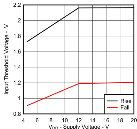
図 7-16. Input Threshold vs Supply Voltage
