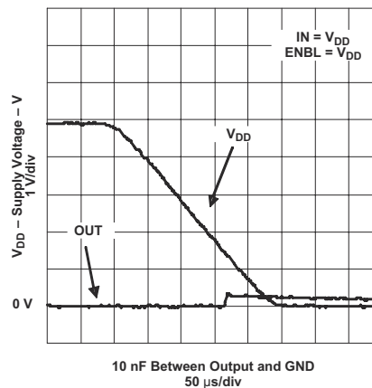
図 7-22. Output Behavior vs VDD (Inverting)
