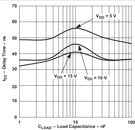
図 7-14. t_{D2} Delay Time vs Load Capacitance
