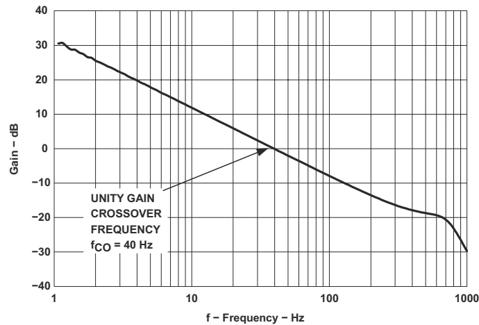
FIG 7-6. Power Module Bode Plot
