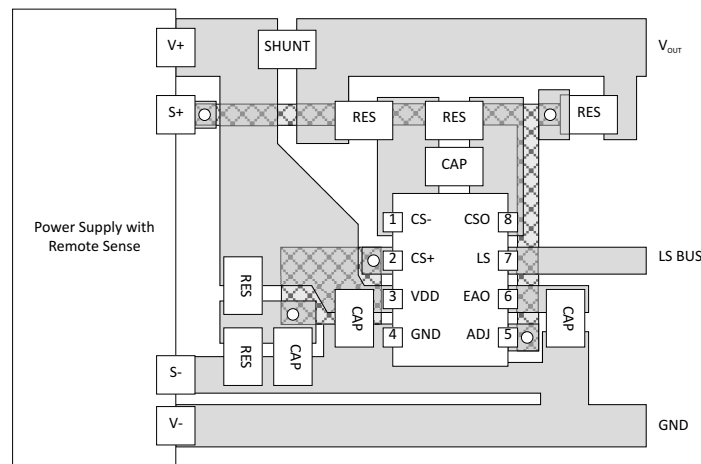
FIG 7-7. Layout Example (2-Layer PCB)
