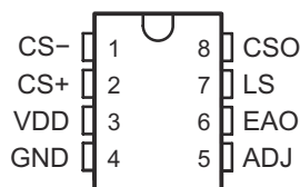
図 4-2. P Package 8-Pin PDIP Top View
