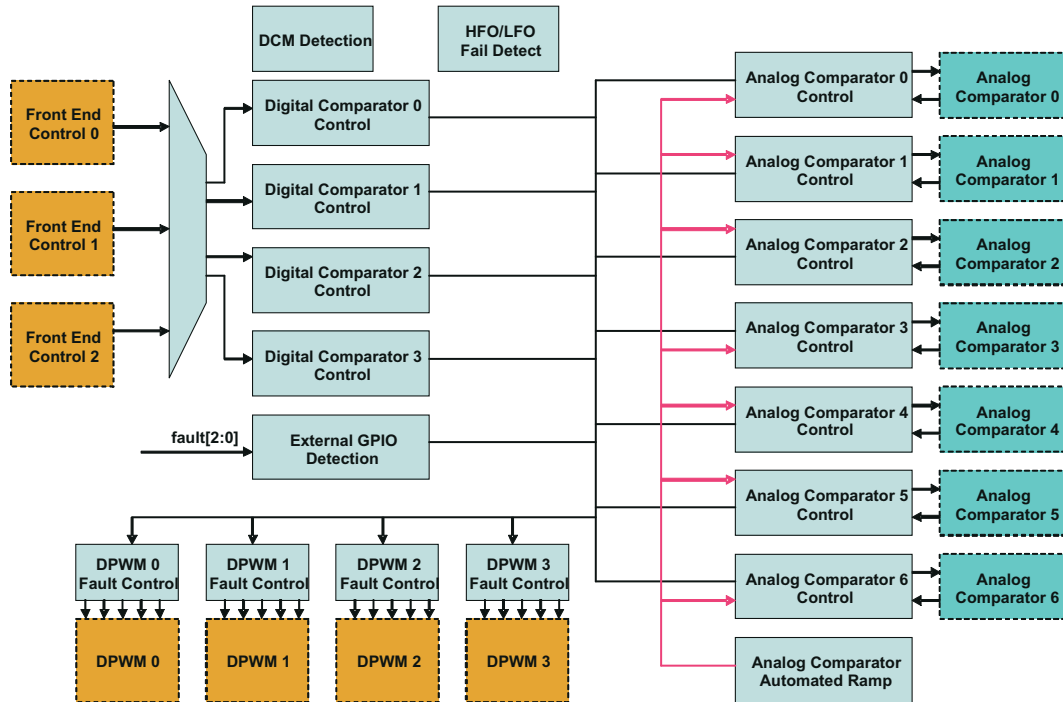
FIG 9-16. Fault Mux Block Diagram
