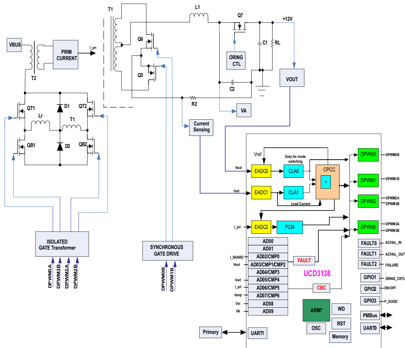
10-1. Phase-Shifted Full-Bridge
