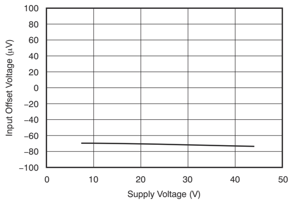
図 5-20. Input Offset Voltage vs Supply Voltage
