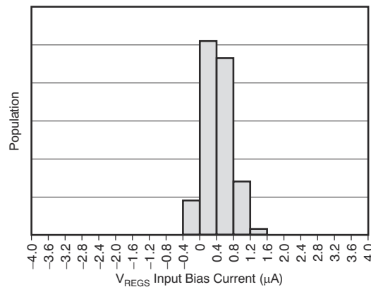
図 5-26. Regulator Input Bias Current Distribution (Current Into REGS Pin)
