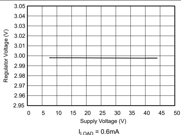
図 5-28. Regulator Voltage vs Supply Voltage
