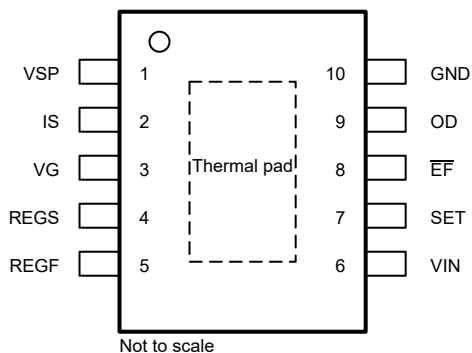
図 4-1. DGQ Package, 10-Pin HVSSOP (Top View)
