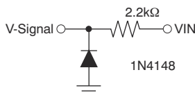
Figure 7-1. Enhanced Protection Against Negative Overload of V_{IN}
