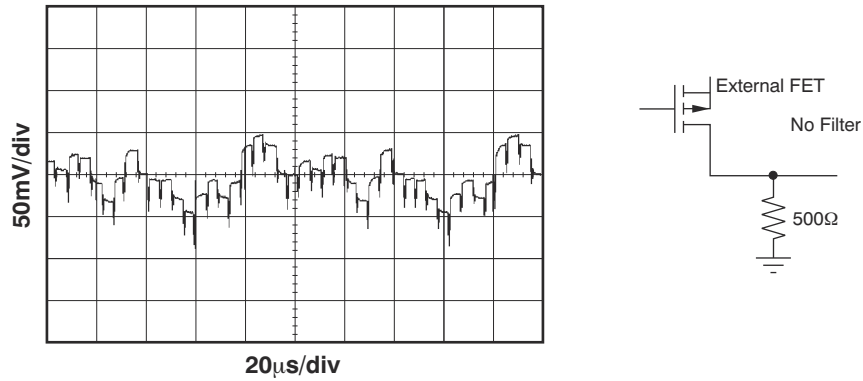
Figure 6-2. Output Noise Without Filter Into 500 \Omega
