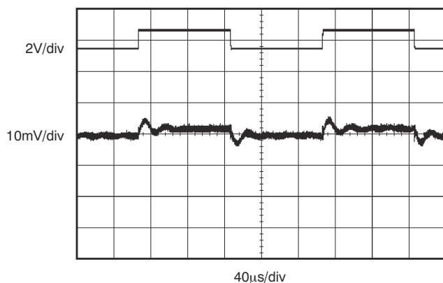
图 5-31. Step Response
