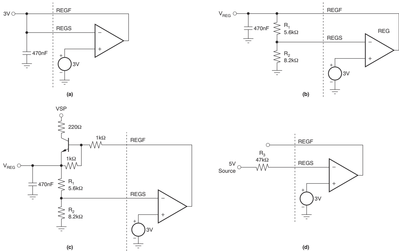
図 6-7. Basic Connections of the Voltage Regulator
