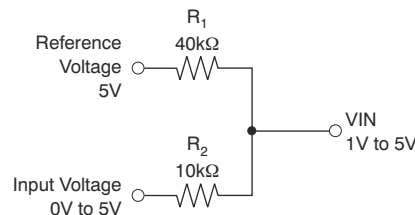
図 7-3. Resistive Divider for I_{MIN} -to- I_{MAX} Output (4mA to 20mA) With 0V to V_{FS} Signal Source
