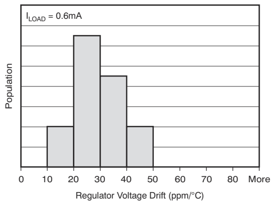
図 5-25. Regulator Voltage Drift Distribution
