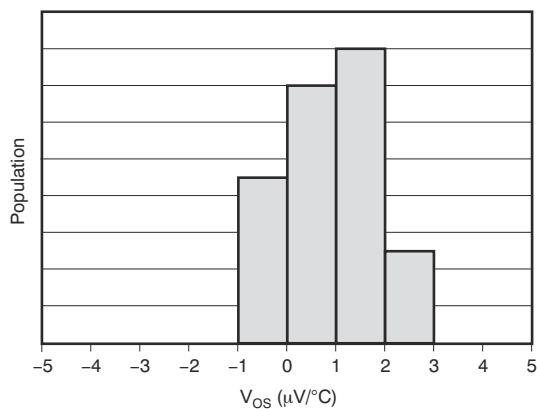
図 5-19. Input Offset Voltage Drift Distribution
