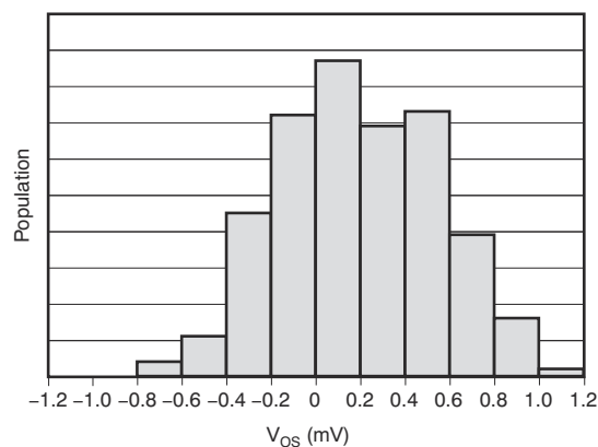
Figure 5-18. Input Offset Voltage Distribution
