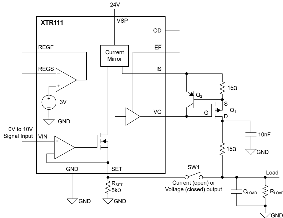
図 7-2. 0V-to-10V or 0mA-to-20mA Output Selected by Jumper SW1
