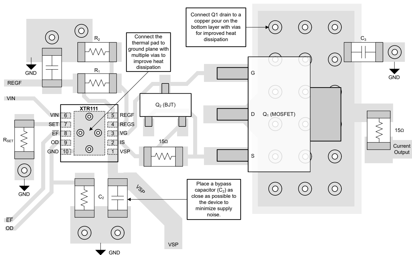
7-8. Layout Example
