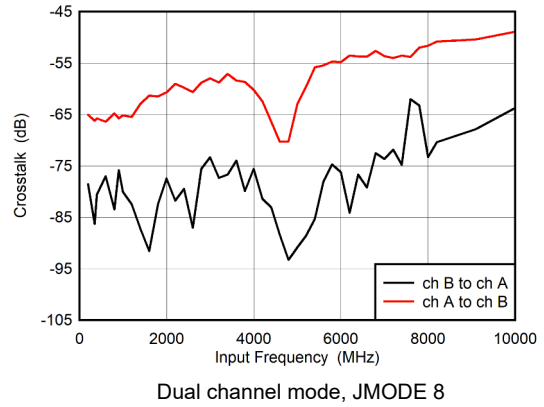
5-2. Crosstalk vs Input Frequency
