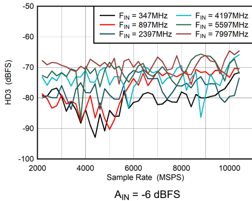
5-39. DES Mode: HD3 vs Sample Rate
