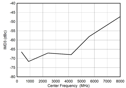
5-100. DES Mode: IMD3 vs Input Frequency
