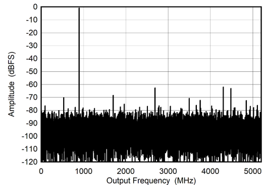
5-6. DES Mode: Single Tone FFT at 897 MHz
