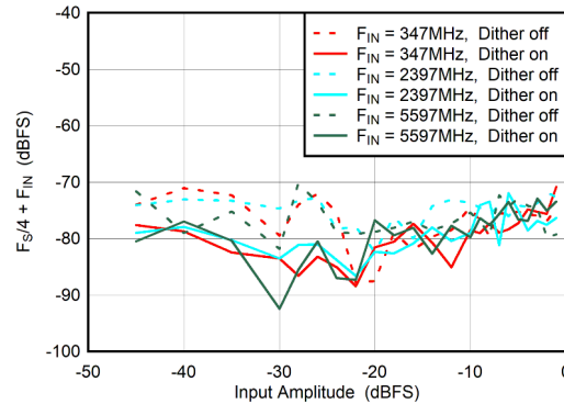
Figure 5-68. DES Mode: F_S/4 + F_{IN} vs Input Amplitude and Dither
