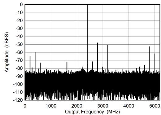
5-10. DES Mode: Single Tone FFT at 7997 MHz
