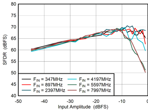
5-73. Dual Channel Mode: SFDR vs Input Amplitude
