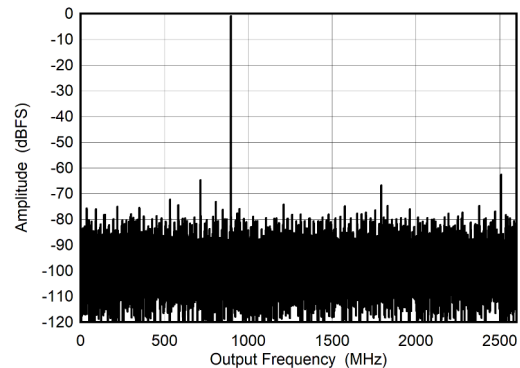
5-18. Dual Channel Mode: Single Tone FFT at 897 MHz
