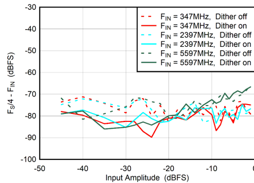
Figure 5-70. DES Mode: F_S/4 - F_{IN} vs Input Amplitude and Dither
