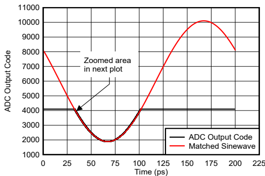
5-125. Sinewave Overdrive Recovery
