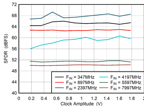
5-84. Dual Channel Mode: SFDR vs Clock Amplitude
