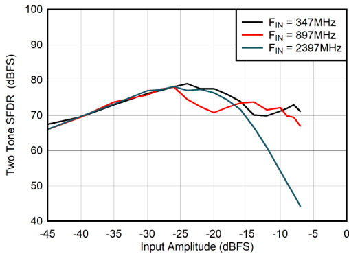
5-109. Dual Channel Mode: Two Tone SFDR vs Input Amplitude
