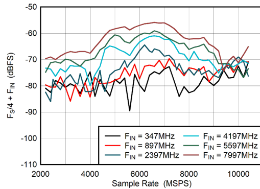
5-42. DES Mode: F_S/4 + F_{IN} vs Sample Rate
