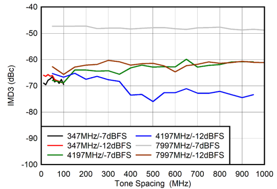
5-102. DES Mode: IMD3 vs Tone Spacing
