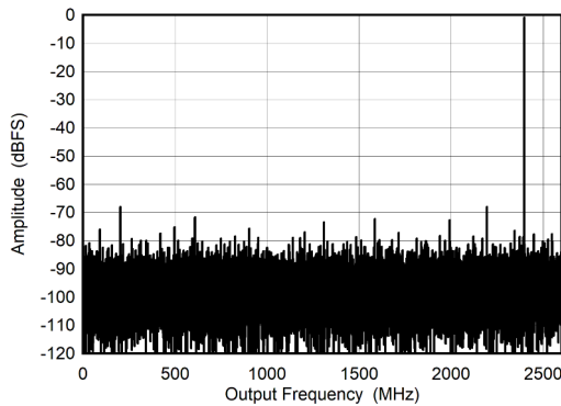
5-19. Dual Channel Mode: Single Tone FFT at 2397 MHz
