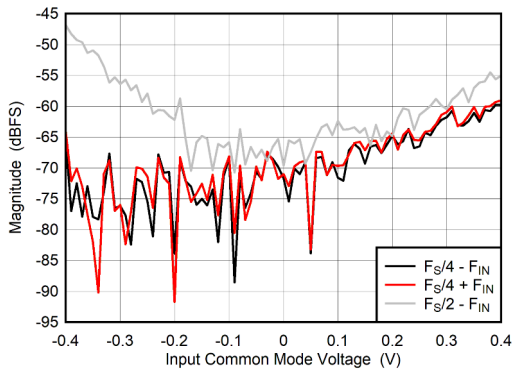
5-99. DES Mode: F_S/2 - F_{\text{IN}} , F_S/4 \pm F_{\text{IN}} vs Input Common Mode Voltage
