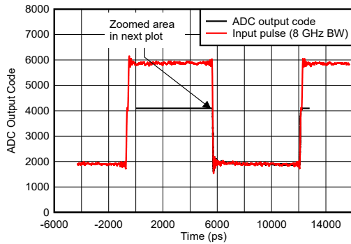
5-123. Pulse Overdrive Recovery
