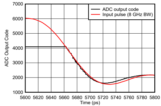
5-124. Pulse Overdrive Recovery Zoomed
