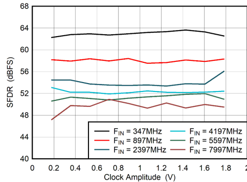
5-82. DES Mode: SFDR vs Clock Amplitude
