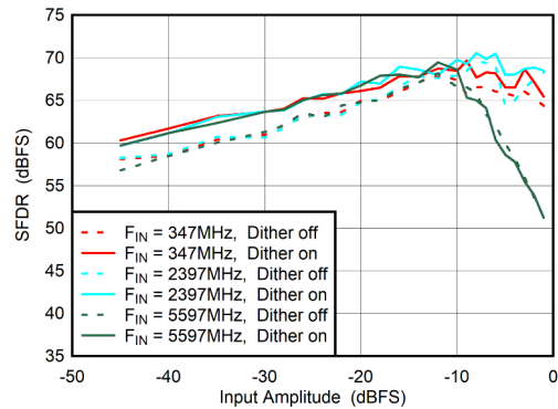
5-74. Dual Channel Mode: SFDR vs Input Amplitude and Dither
