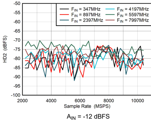
5-37. DES Mode: HD2 vs Sample Rate
