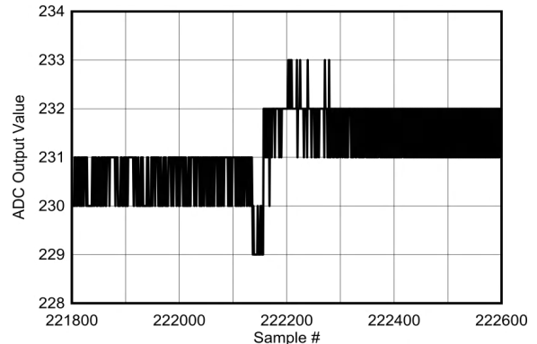
5-122. Background Calibration Core Transition (DC Signal Zoomed)
