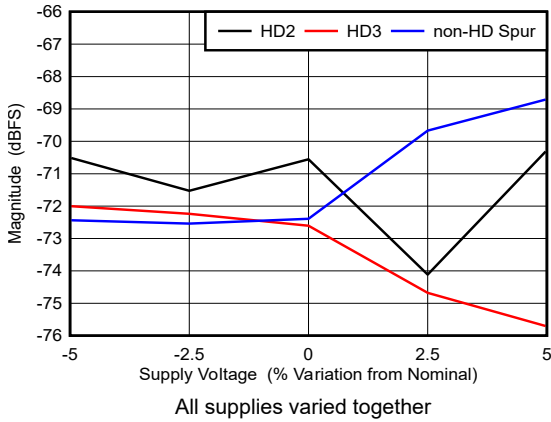
5-97. Dual Channel Mode: HD2, HD3 and Worst Spur vs Supply Voltage
