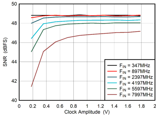
5-81. DES Mode: SNR vs Clock Amplitude
