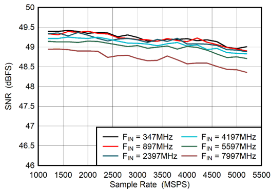
5-45. Dual Channel Mode: SNR vs Sample Rate
