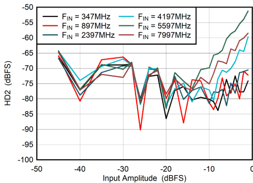
5-75. Dual Channel Mode: HD2 vs Input Amplitude
