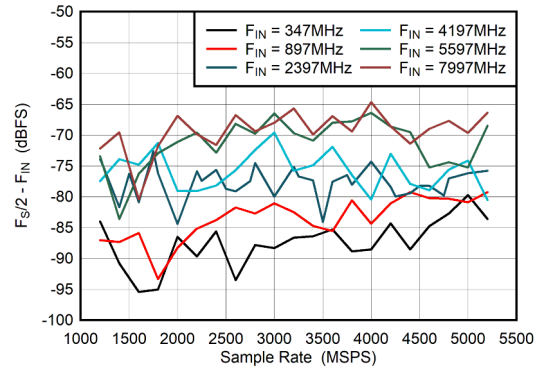
5-56. Dual Channel Mode: F_S/2 - F_{IN} vs Sample Rate
