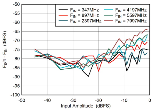
Figure 5-69. DES Mode: F_S/4 - F_{IN} vs Input Amplitude
