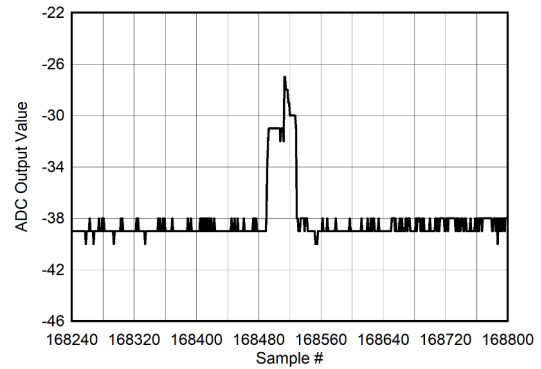
5-120. Background Calibration Core Transition (AC Signal Zoomed)
