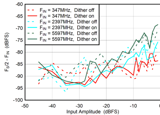
5-80. Dual Channel Mode: F_{S/2} - F_{IN} vs Input Amplitude and Dither
