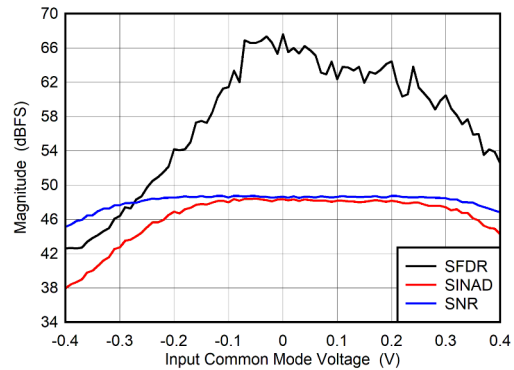
5-98. DES Mode: SNR, SFDR and SINAD vs Input Common Mode Voltage
