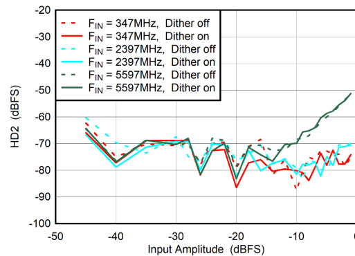
5-76. Dual Channel Mode: HD2 vs Input Amplitude and Dither
