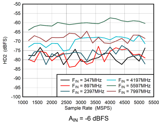
5-51. Dual Channel Mode: HD2 vs Sample Rate
