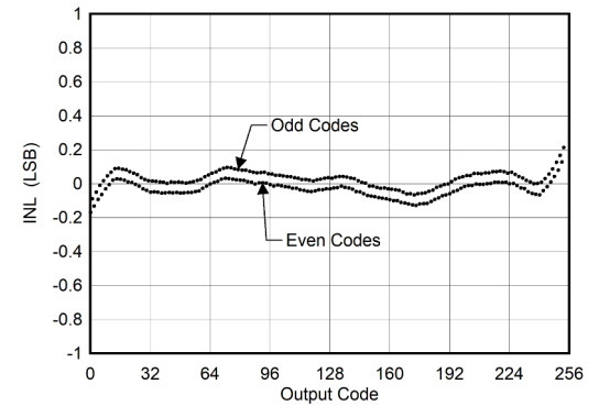
5-4. INL vs ADC Code
