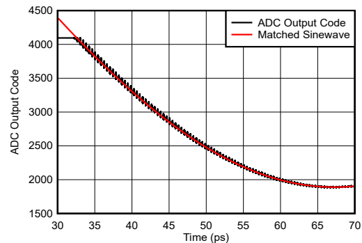
5-126. Sinewave Overdrive Recovery
