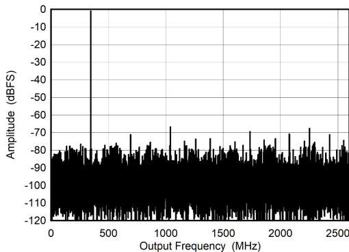
5-17. Dual Channel Mode: Single Tone FFT at 347 MHz
