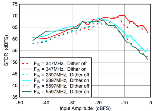
5-60. DES Mode: SFDR vs Input Amplitude and Dither
