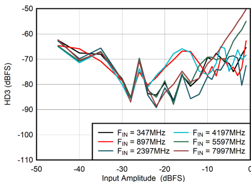
5-77. Dual Channel Mode: HD3 vs Input Amplitude
