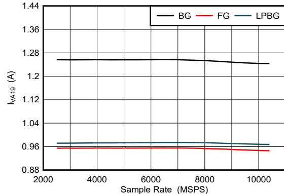
5-110. DES Mode: I_{VA19} vs Sample Rate
