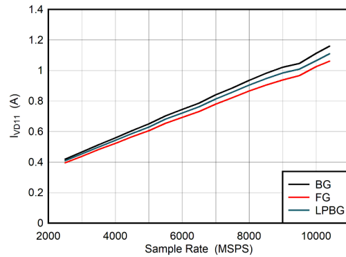
5-112. DES Mode: I_{VD11} vs Sample Rate
