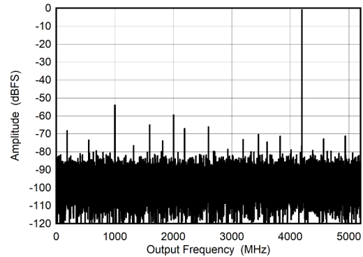
5-8. DES Mode: Single Tone FFT at 4197 MHz
