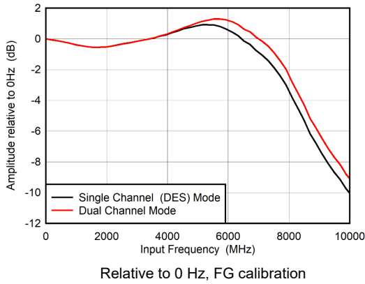
5-1. Input Amplitude vs Input Frequency
