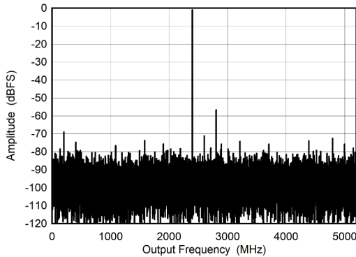
5-7. DES Mode: Single Tone FFT at 2397 MHz
