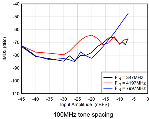
5-101. DES Mode: IMD3 vs Input Amplitude
