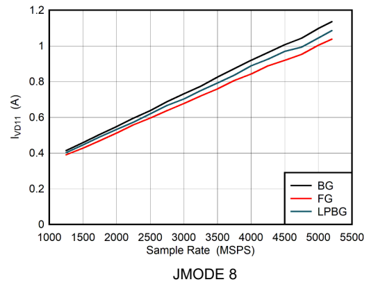
5-116. Dual Channel Mode: I_{V_{D11}} vs Sample Rate
