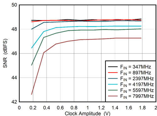
5-83. Dual Channel Mode: SNR vs Clock Amplitude
