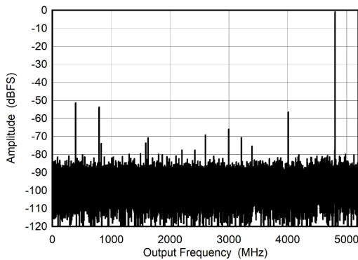
5-9. DES Mode: Single Tone FFT at 5597 MHz
