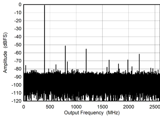
5-21. Dual Channel Mode: Single Tone FFT at 5597 MHz
