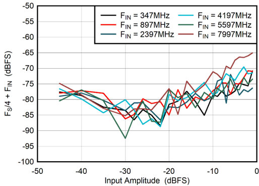
Figure 5-67. DES Mode: F_S/4 + F_{IN} vs Input Amplitude
