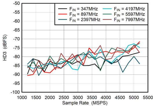
5-55. Dual Channel Mode: HD3 vs Sample Rate
