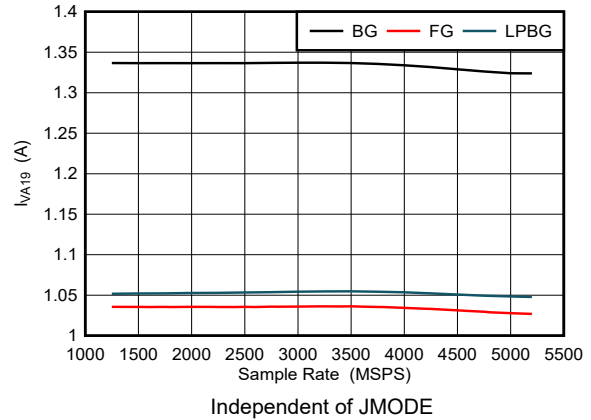
5-114. Dual Channel Mode: I_{V_{A19}} vs Sample Rate
