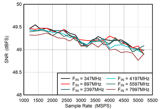
5-44. Dual Channel Mode: SNR vs Sample Rate
