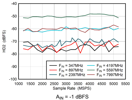
5-50. Dual Channel Mode: HD2 vs Sample Rate
