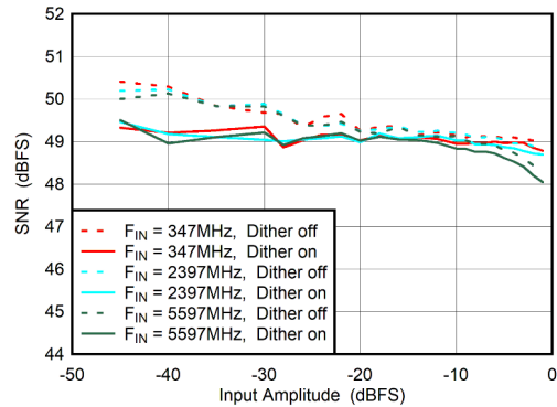
5-58. DES Mode: SNR vs Input Amplitude and Dither
