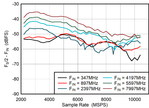
5-41. DES Mode: F_S/2 - F_{IN} vs Sample Rate
