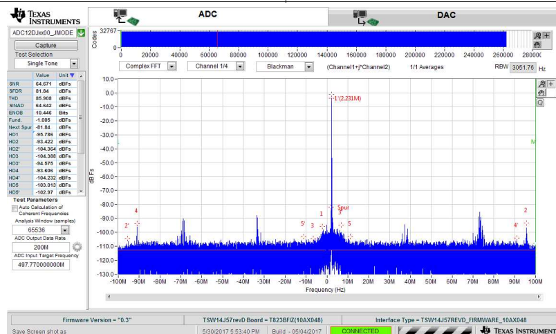
181. FFT for 497.77-MHz Input Signal, 6.4 GSPS, JMODE0
