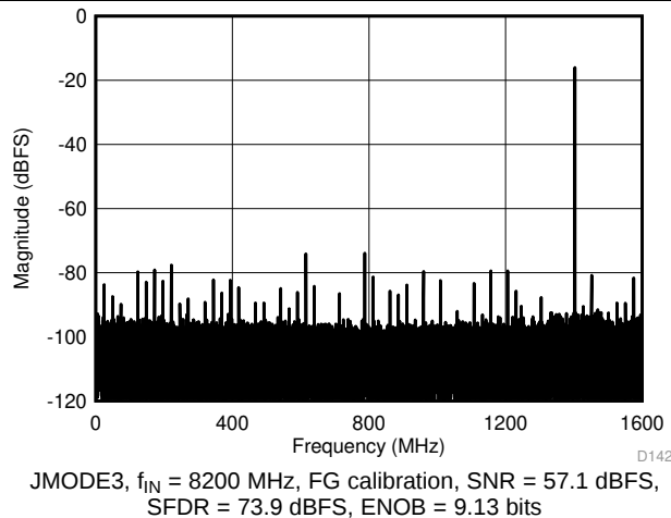
Figure 28. Single-Tone FFT at A_{\text{IN}} = -16\text{ dBFS}
