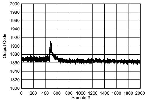
6-138. Background Calibration Core Transition (DC Offset Signal)
