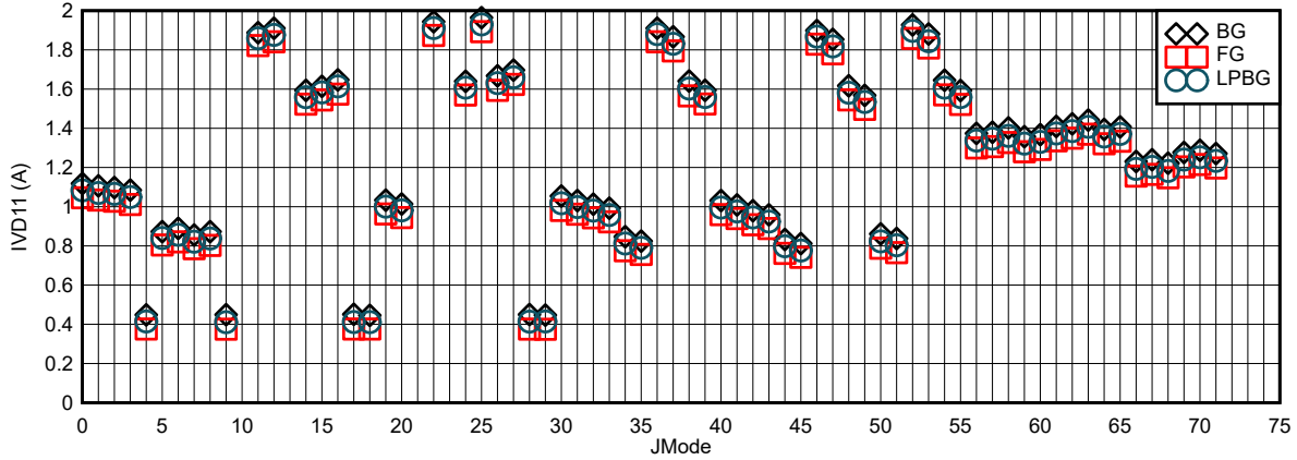
6-115. I_{VD11} vs \text{JMODE} at F_{\text{CLK}} = 4\text{ GHz}
