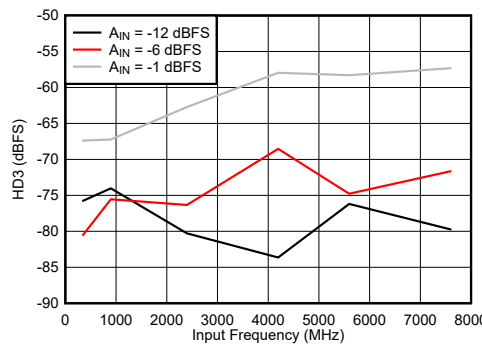
6-80. DES Mode: HD3 vs Input Frequency
