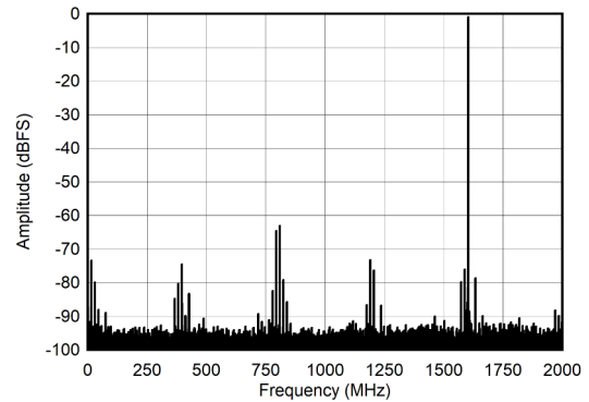
6-20. Dual Channel Mode: Single Tone FFT at 2397 MHz
