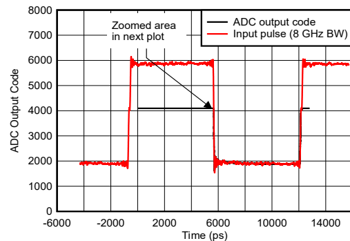
6-141. Pulse Overdrive Recovery
