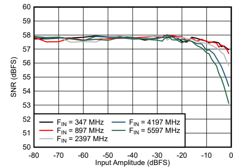
Figure 6-55. DES Mode: SNR vs Input Amplitude and Frequency
