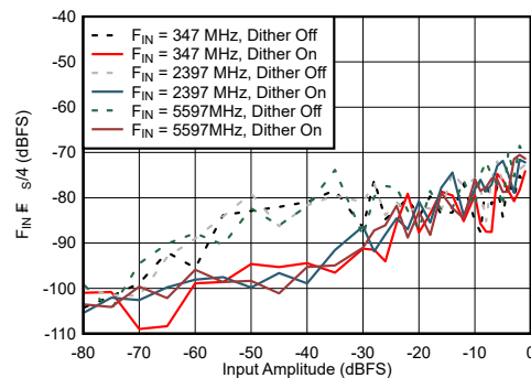
Figure 6-66. DES Mode: F_{IN} \pm F_{IN}/4 vs Input Amplitude and Dither
