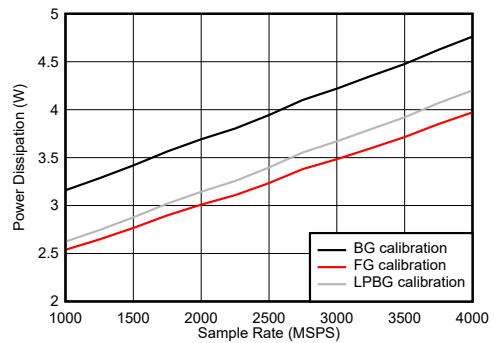
图 6-123. DES Mode: Power Dissipation vs Sample Rate
