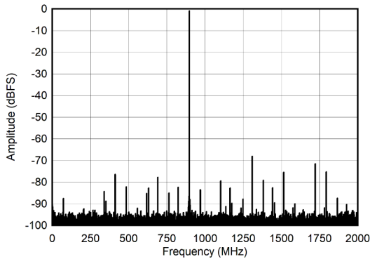
6-19. Dual Channel Mode: Single Tone FFT at 897 MHz
