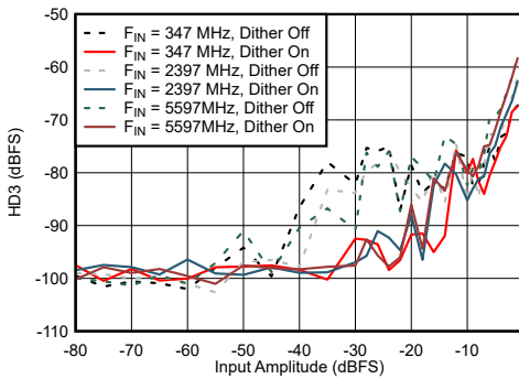
Figure 6-62. DES Mode: HD3 vs Input Amplitude and Dither
