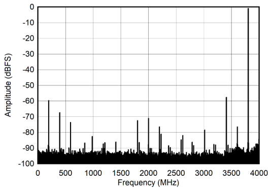
6-11. DES Mode: Single Tone FFT at 4197 MHz
