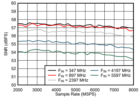
Figure 6-28. DES Mode: SNR vs Sample Rate and Input Frequency
