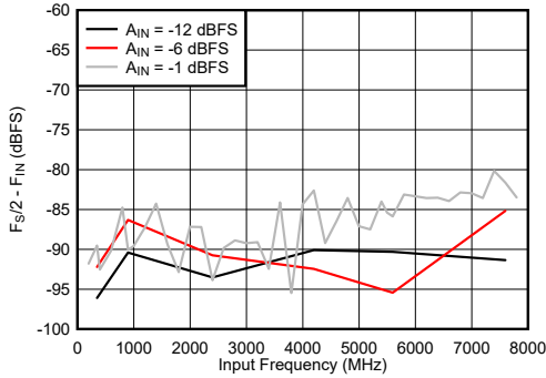
Figure 6-87. Dual Channel Mode: F_S/2 - F_{IN} vs Input Frequency
