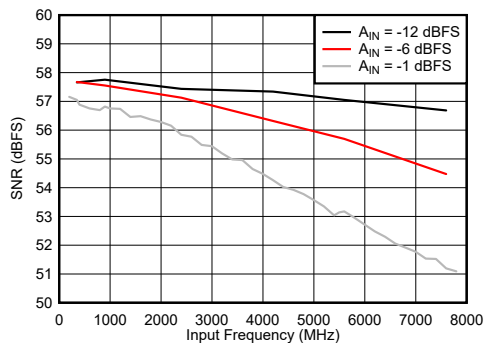
6-83. Dual Channel Mode: SNR vs Input Frequency
