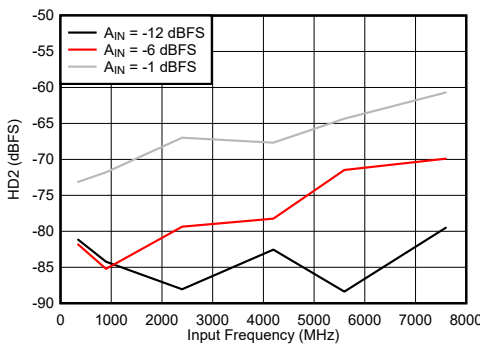
6-79. DES Mode: HD2 vs Input Frequency
