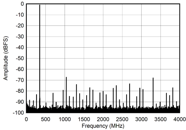
8-2. FFT for 347 MHz Input Signal, 8 GSPS, JMODE1
