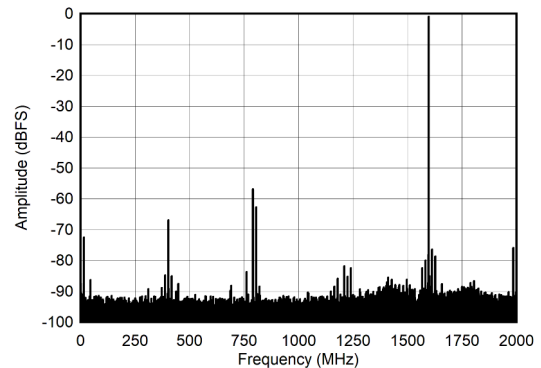
6-22. Dual Channel Mode: Single Tone FFT at 5597 MHz
