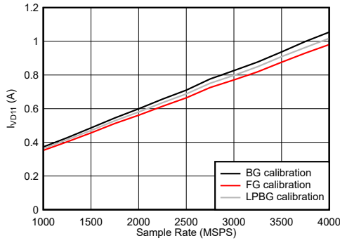
图 6-120. DES Mode: I_{VD11} vs Sample Rate
