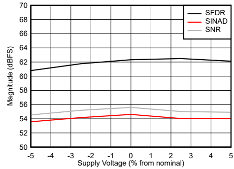
6-100. DES Mode: SNR, SINAD and SFDR vs Supply Voltage
