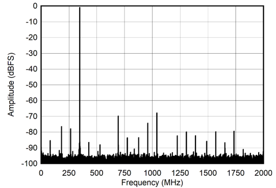
6-18. Dual Channel Mode: Single Tone FFT at 347 MHz
