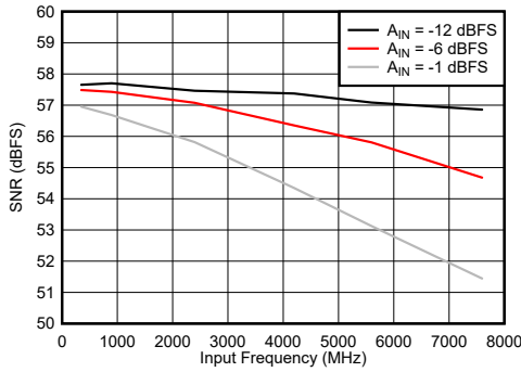
6-77. DES Mode: SNR vs Input Frequency
