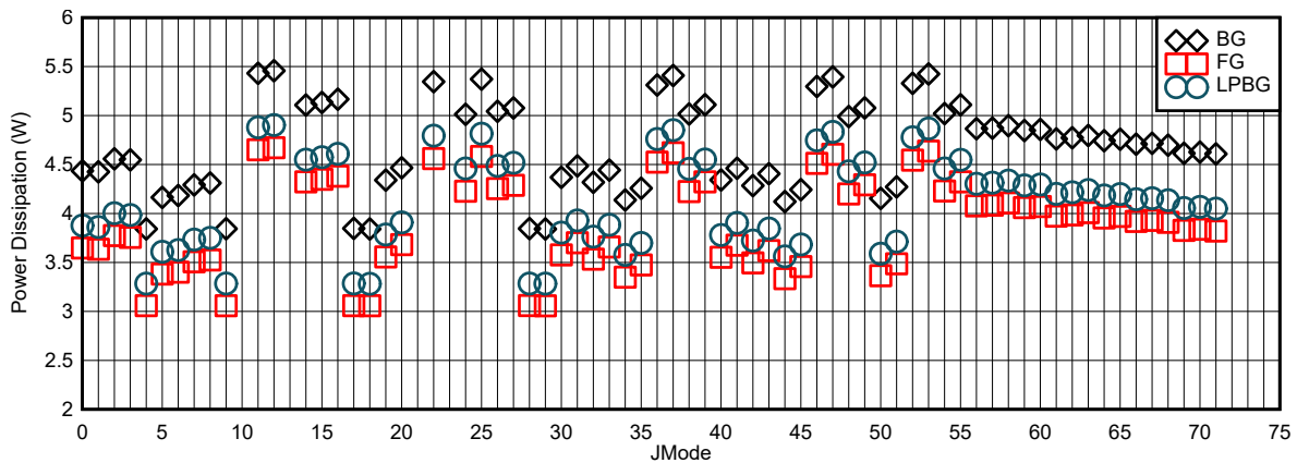
图 6-114. Power Dissipation vs JMODE at F_{CLK} = 4\text{ GHz}
