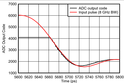
6-142. Pulse Overdrive Recovery Zoomed
