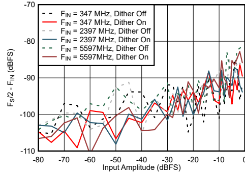
6-76. Dual Channel Mode: F_S/2 - F_{IN} vs Input Amplitude and Dither
