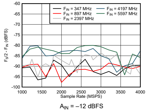
Figure 6-54. Dual Channel Mode: F_S/2 - F_{\text{IN}} vs Sample Rate and Input Frequency
