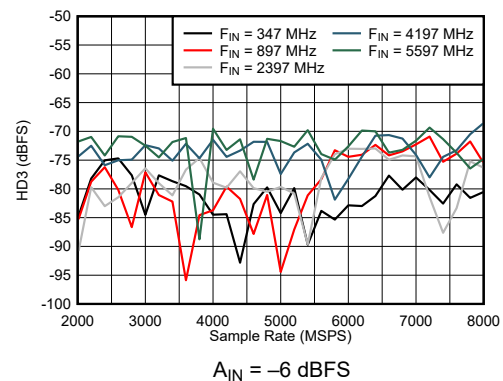
图 6-38. DES Mode: HD3 vs Sample Rate and Input Frequency
