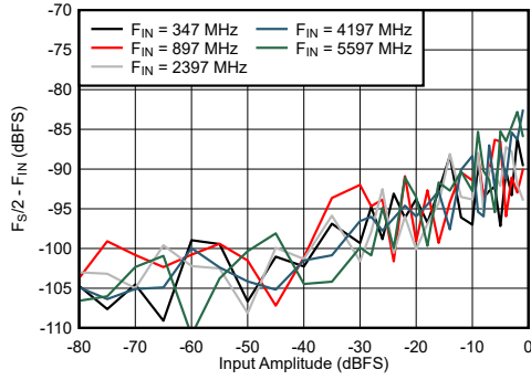
6-75. Dual Channel Mode: F_S/2 - F_{IN} vs Input Amplitude and Frequency
