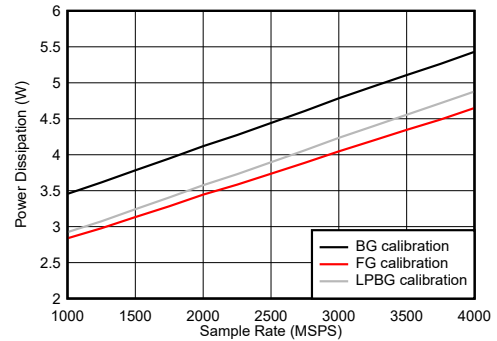
6-133. Dual Channel Mode: Power Dissipation vs Sample Rate
