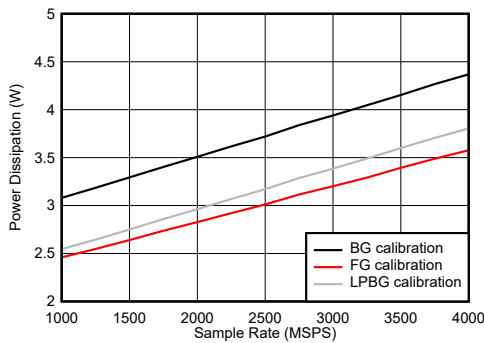
图 6-122. DES Mode: Power Dissipation vs Sample Rate
