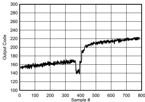
6-140. Background Calibration Core Transition (AC Signal Zoomed)
