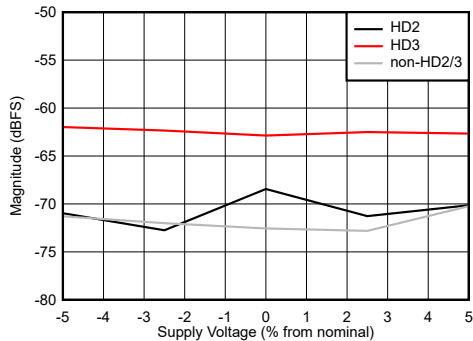
6-101. DES Mode: HD2, HD3 and Worst non-HD Spur vs Supply Voltage
