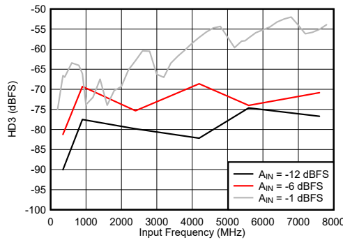
6-86. Dual Channel Mode: HD3 vs Input Frequency
