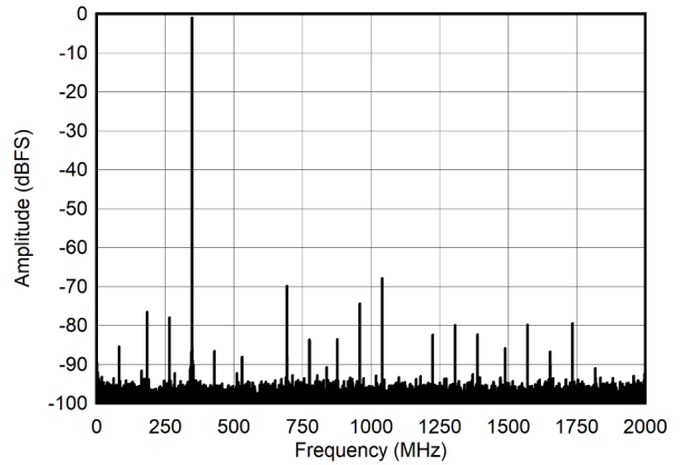
8-3. FFT for 347 MHz Input Signal, 4 GSPS, JMODE3
