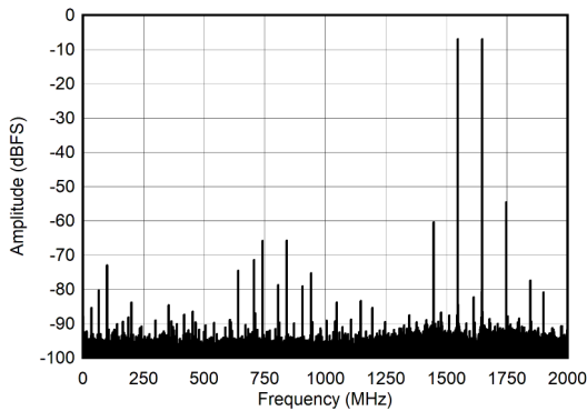
Figure 6-27. Dual Channel Mode: Two Tone FFT at 4197 MHz
