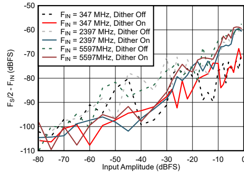
Figure 6-64. DES Mode: F_S/2 - F_{IN} vs Input Amplitude and Dither
