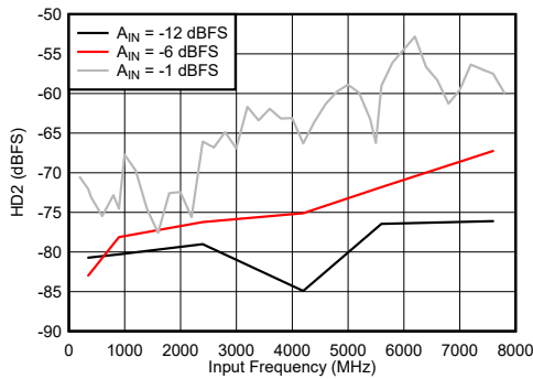
6-85. Dual Channel Mode: HD2 vs Input Frequency
