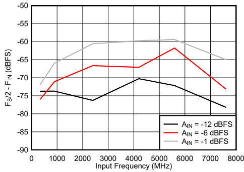
6-81. DES Mode: F_S/2 - F_{IN} vs Input Frequency
