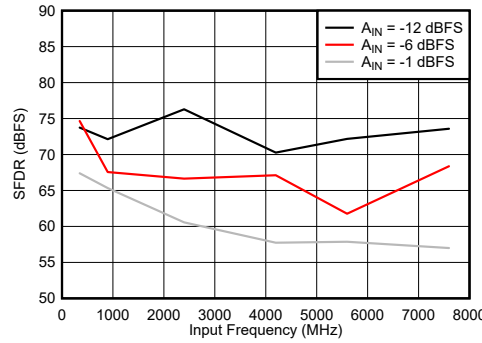
6-78. DES Mode: SFDR vs Input Frequency
