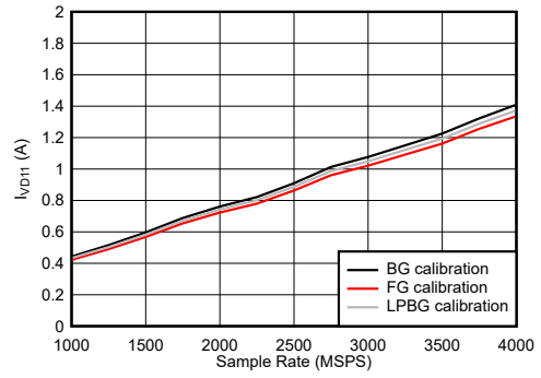
图 6-121. DES Mode: I_{VD11} vs Sample Rate
