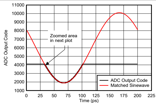
6-143. Sinewave Overdrive Recovery
