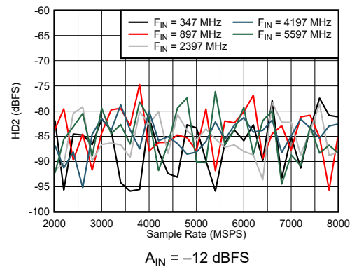
图 6-36. DES Mode: HD2 vs Sample Rate and Input Frequency
