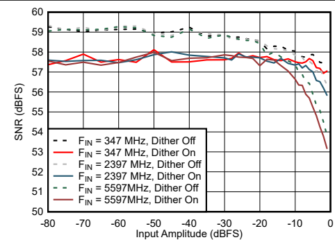
Figure 6-68. Dual Channel Mode: SNR vs Input Amplitude and Dither
