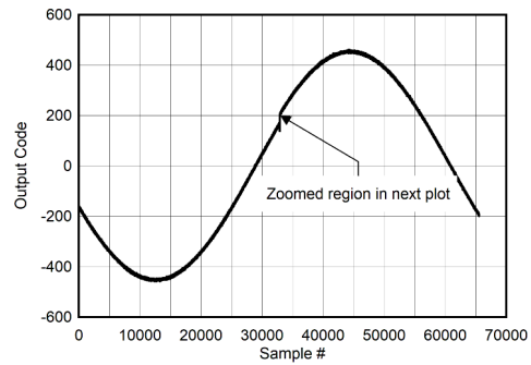
6-139. Background Calibration Core Transition (AC Signal)
