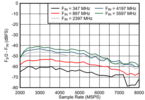
Figure 6-40. DES Mode: F_S/2 - F_{IN} vs Sample Rate and Input Frequency
