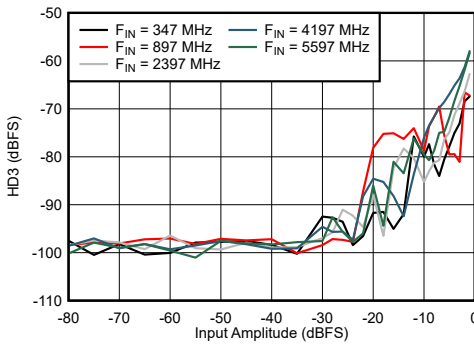
Figure 6-61. DES Mode: HD3 vs Input Amplitude and Frequency
