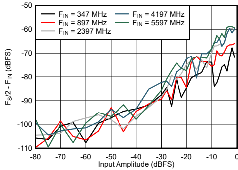
Figure 6-63. DES Mode: F_S/2 - F_{IN} vs Input Amplitude and Frequency
