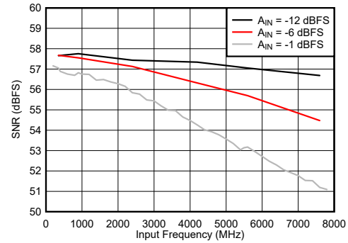
6-82. DES Mode: F_{IN} \pm F_S/4 vs Input Frequency
