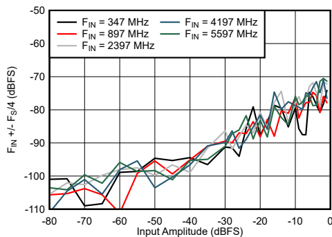
Figure 6-65. DES Mode: F_{IN} \pm F_{IN}/4 vs Input Amplitude and Frequency
