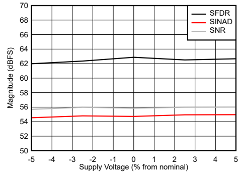
6-102. Dual Channel Mode: SNR, SINAD and SFDR vs Supply Voltage
