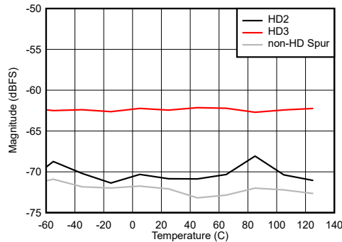
FG calibration at each temperature
