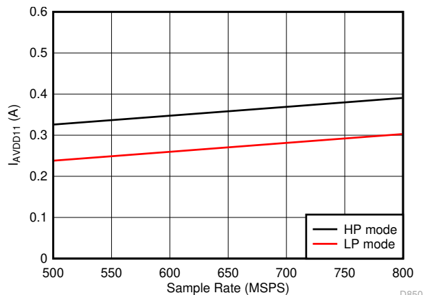
Figure 5-93. Dual Channel, I_{VA11} vs F_S
