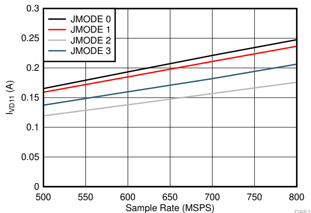
Figure 5-94. Dual Channel, I_{VD11} vs F_S for JMODES 0 - 3
