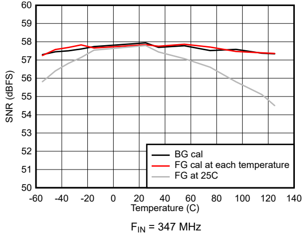
Figure 5-43. SNR vs Temperature
