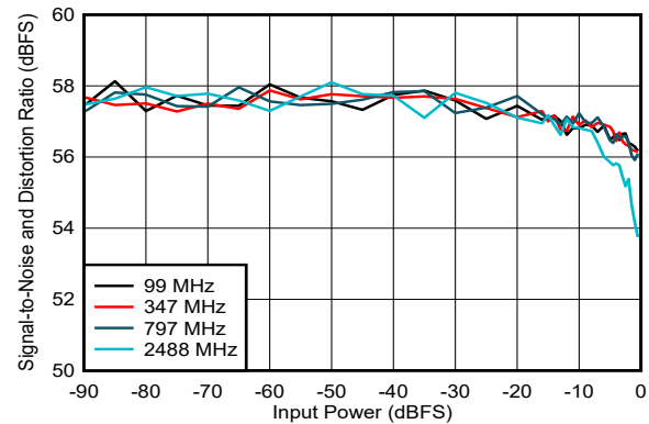
Figure 5-119. SNR vs Input Power
