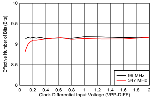
5-34. ENOB vs Clock Amplitude
