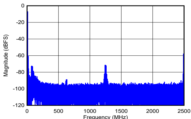
FIG 5-261. Two-Tone FFT at f_{IN} = 2488\text{MHz} , A_{IN} = -1\text{dBFS}
