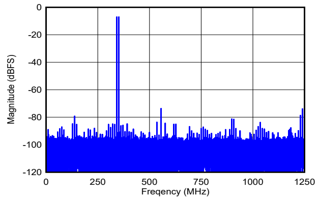
DES_EN = 0, f_S = 2500\text{MHz} , FG calibration, f_1 = 342\text{MHz} , f_2 = 352\text{MHz} , A_{IN} = -7\text{dBFS} per tone, SFDR = -74dBFS, IMD3 = -86dBFS, IMD2 = -88dBFS
