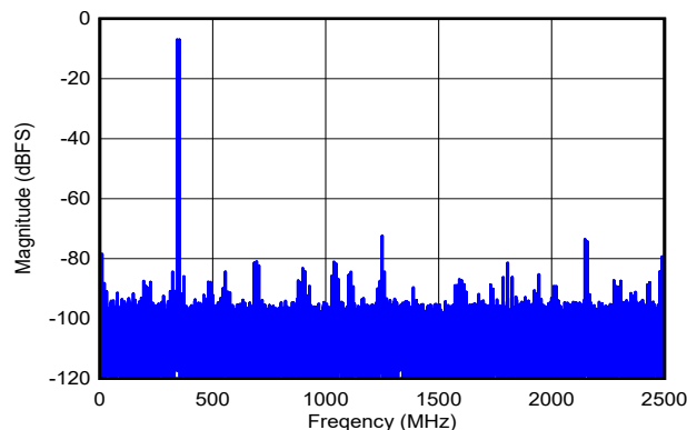
DES_EN = 1, f_S = 5000\text{MHz} , FG calibration, f_1 = 342\text{MHz} , f_2 = 352\text{MHz} , A_{IN} = -7\text{dBFS} per tone, SFDR = -74dBFS, IMD3 = -91dBFS, IMD2 = -80dBFS
