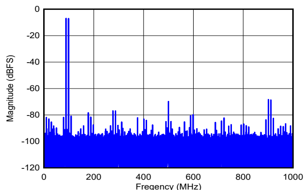
DES_EN = 1, f_S = 2000\text{MHz} , FG calibration, f_1 = 89\text{MHz} , f_2 = 99\text{MHz} , A_{IN} = -7\text{dBFS} per tone, SFDR = -68dBFS, IMD3 = -81dBFS, IMD2 = -82dBFS
