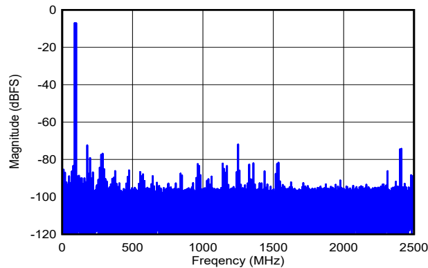
DES_EN = 1, f_S = 5000\text{MHz} , FG calibration, f_1 = 89\text{MHz} , f_2 = 99\text{MHz} , A_{IN} = -7\text{dBFS} per tone, SFDR = -72dBFS, IMD3 = -86dBFS, IMD2 = -86dBFS
