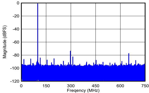
FIG 5-134. Single-Tone FFT at f_{IN} = 99\text{MHz} , A_{IN} = -1\text{dBFS}
