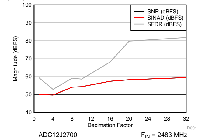
Figure 9. SNR, SINAD, SFDR vs Decimation Setting
