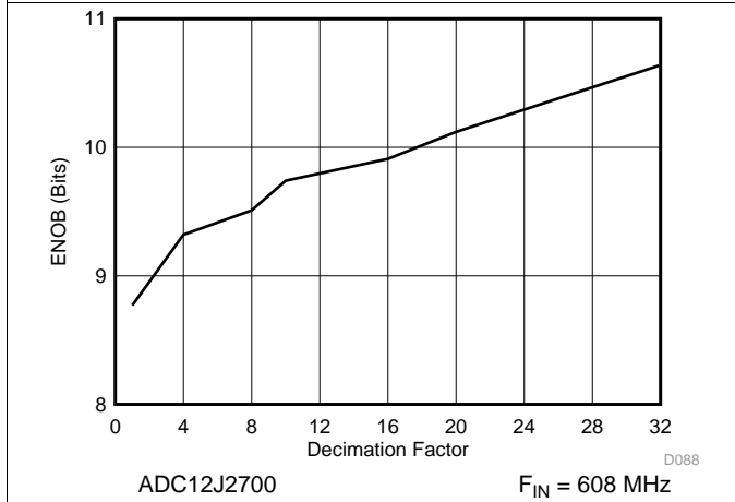
Figure 13. ENOB vs Decimation Setting
