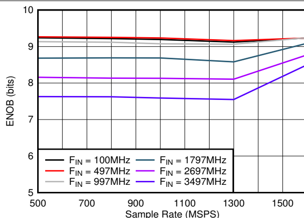
8-26. ENOB vs Sample Rate
