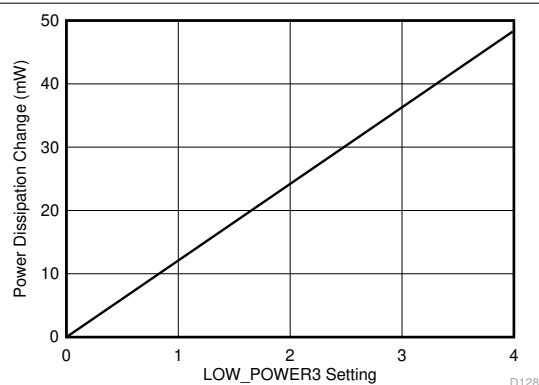
图 9-13. Power Dissipation Change vs LOW_POWER3 register setting
