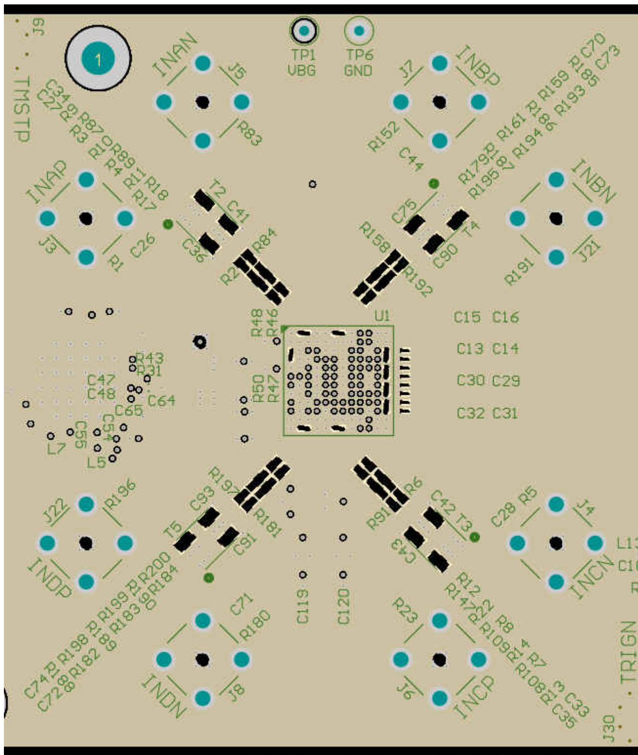
✎ 12-2. GND1 Cutouts to Optimize Impedance of Component Pads
