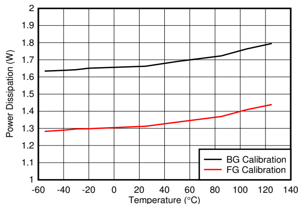
8-121. Quad Channel, Power Dissipation vs Temperature
