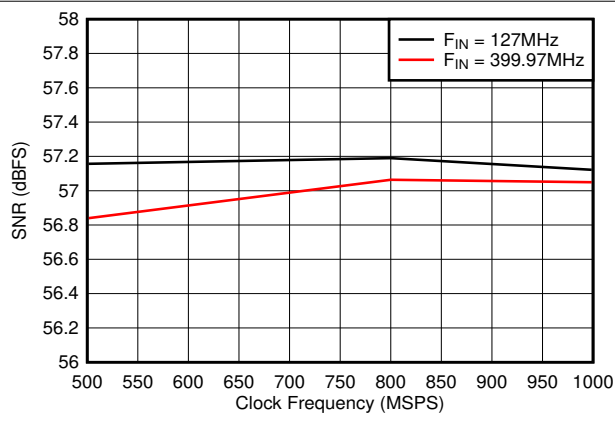
8-28. SNR vs Sample Rate
