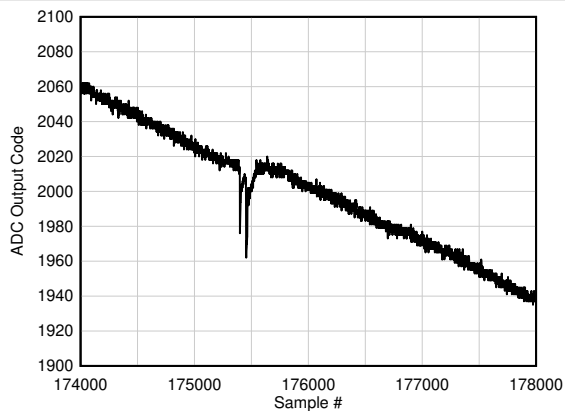
8-127. Background Calibration Core Transition (AC Signal Zoomed)
