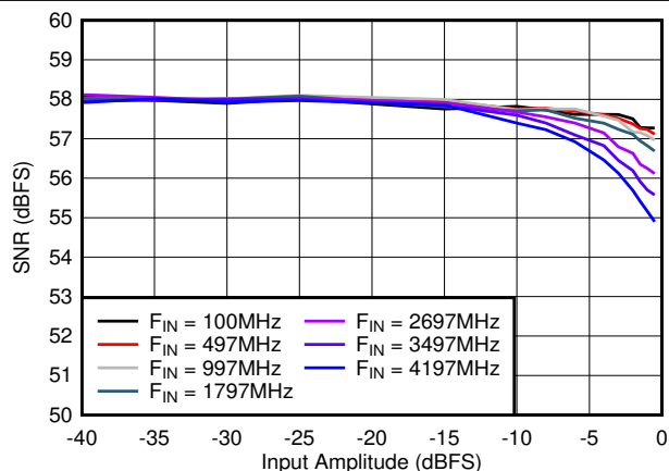
8-33. SNR vs A_{IN}
