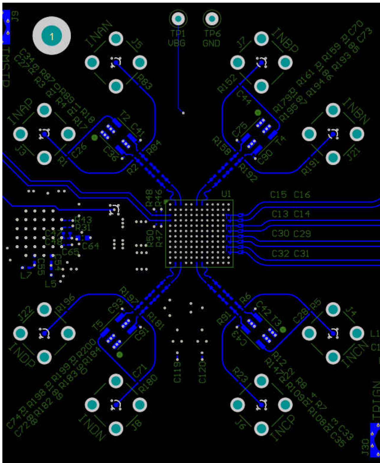
12-1. Top Layer Routing: Analog Inputs (INA±, INB±, INC±, IND±), TMSTP± and D[3:0]± Routing
