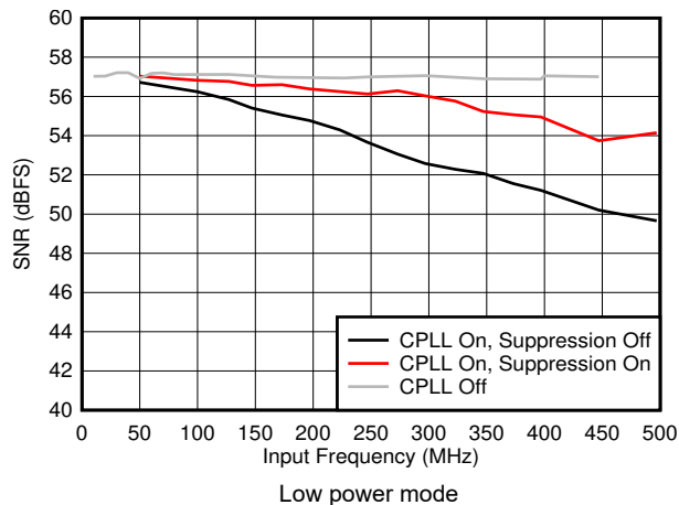
FIG 8-45. SNR vs F_{IN} and C-PLL modes
