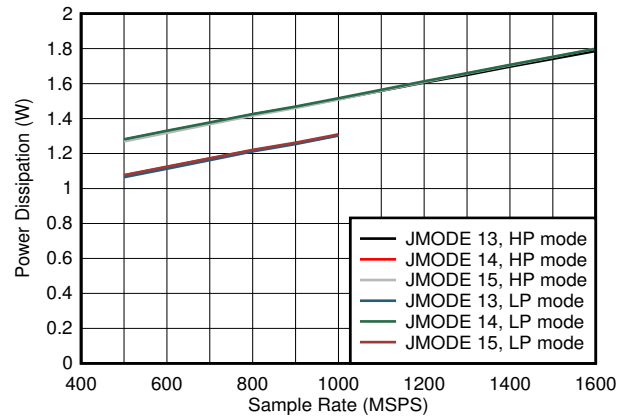
8-92. Dual Channel, Power Dissipation vs F_S and JMODE 13 - 15
