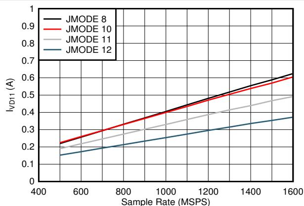
8-87. Quad Channel, I_{VD11} vs F_S and JMODE 8 - 12
