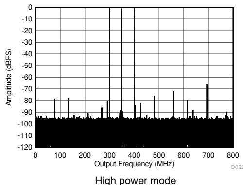
FIG 8-4. Single Tone FFT at 347 MHz and -1 dBFS
