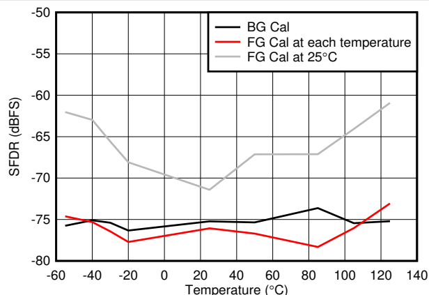
Figure 8-68. Worst Spur vs Temperature
