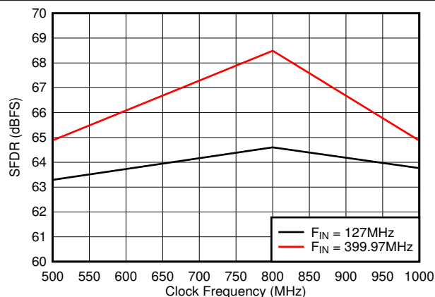
8-27. SFDR vs Sample Rate
