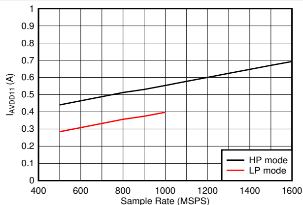
8-84. Quad Channel, I_{VA11} vs F_S
