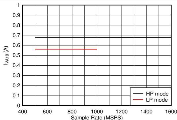
8-83. Quad Channel, I_{VA19} vs F_S
