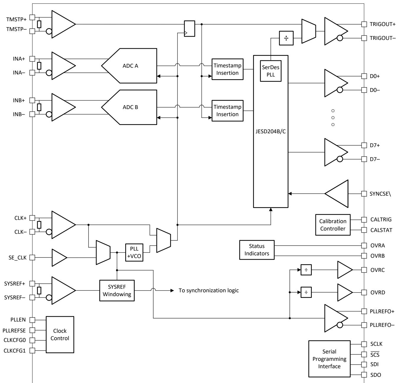
9-2. Dual Channel Functional Block Diagram
