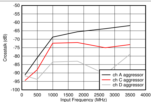
FIG 8-78. Crosstalk to Channel B vs F_{IN}
