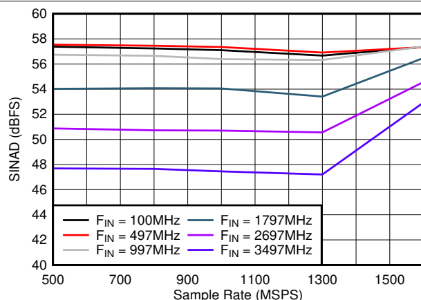
8-25. SINAD vs Sample Rate
