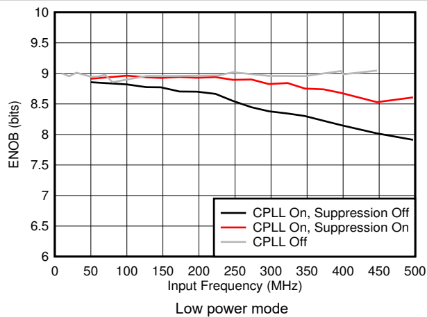
FIG 8-47. ENOB vs F_{IN} and C-PLL modes
