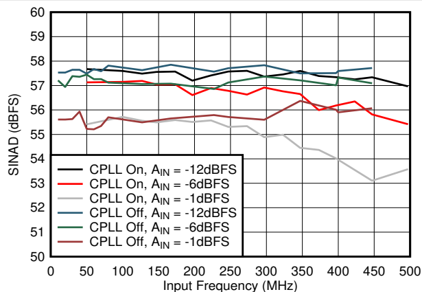
FIG 8-56. SINAD vs A_{IN} and C-PLL
