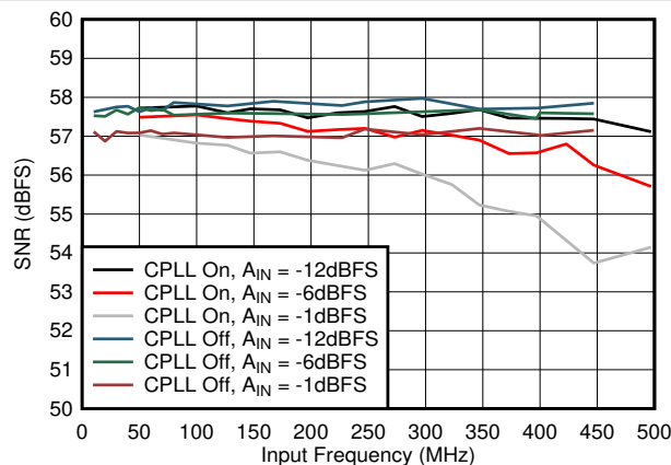
FIG 8-55. SNR vs A_{IN} and C-PLL
