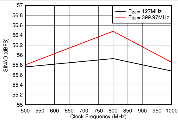
8-30. SINAD vs Sample Rate
