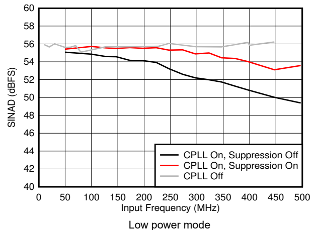
FIG 8-46. SINAD vs F_{IN} and C-PLL modes
