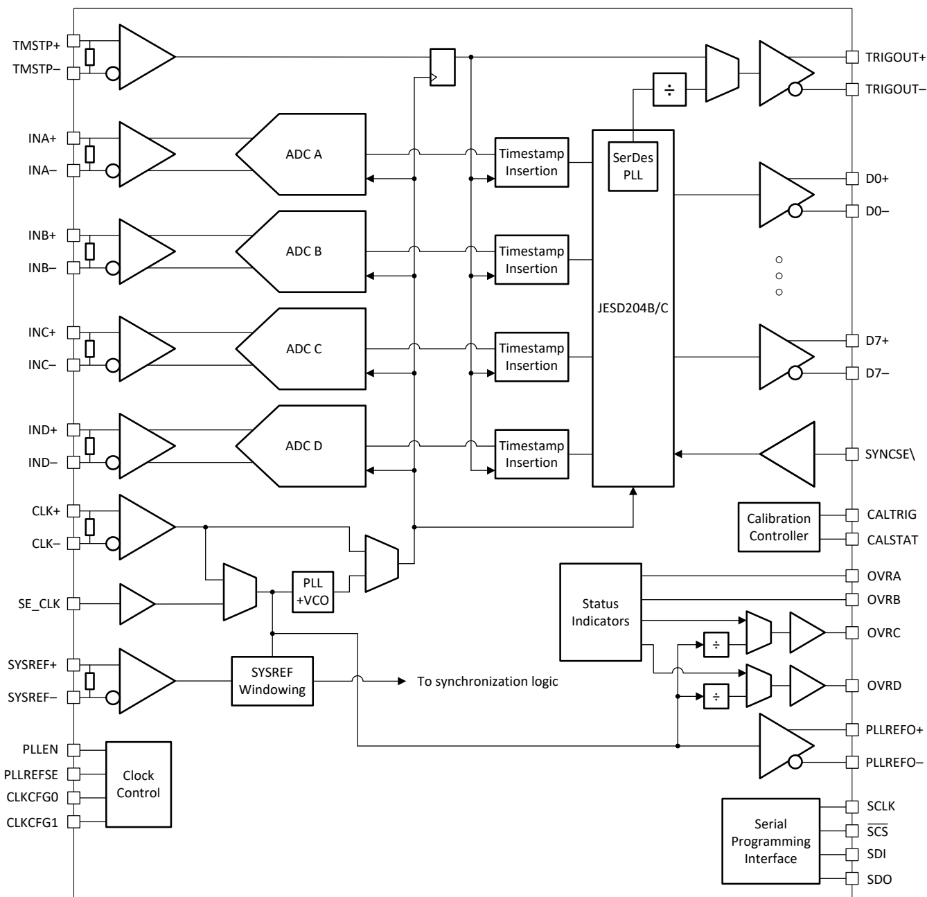
9-1. Quad Channel Functional Block Diagram
