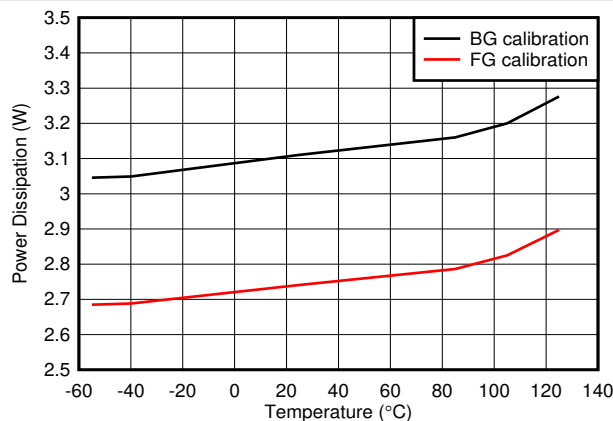
8-121. Quad Channel, Power Dissipation vs Temperature
