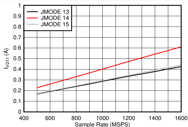
8-88. Quad Channel, I_{VD11} vs F_S and JMODE 13 - 15
