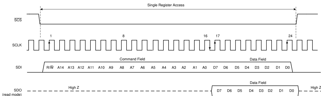
9-18. Serial Interface Protocol: Single Read/Write
