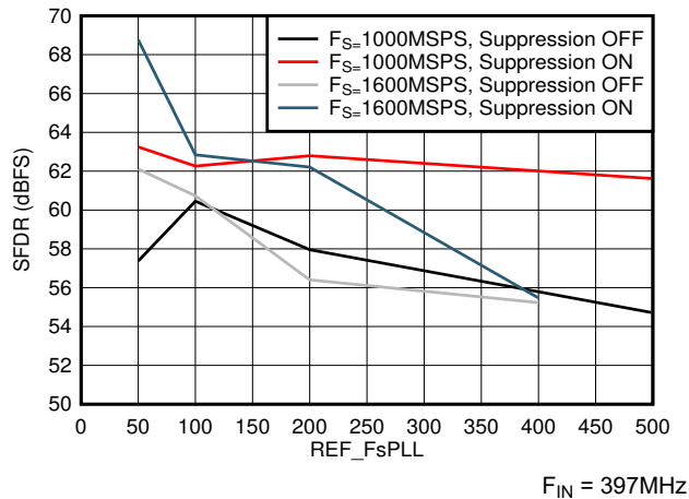
8-39. SFDR vs F_{REF} and Suppression
