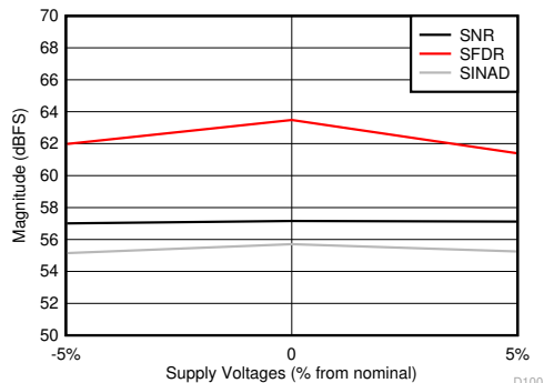
FIG 8-60. SNR, SFDR and SINAD vs Supply Voltage
