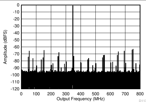
FIG 8-6. Single Tone FFT at 347 MHz and -1 dBFS
