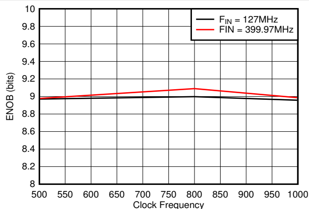
8-31. ENOB vs Sample Rate
