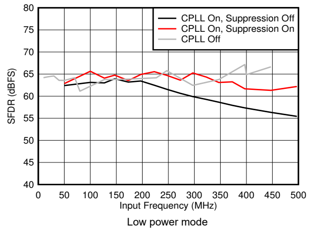
FIG 8-44. SFDR vs F_{IN} and C-PLL modes
