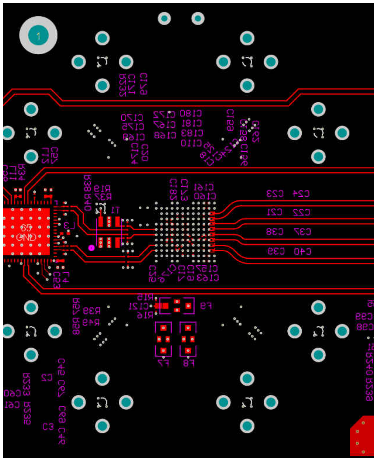
FIG 12-3. Bottom Layer Routing: CLK±, SYSREF and D[7:4]± Routing
