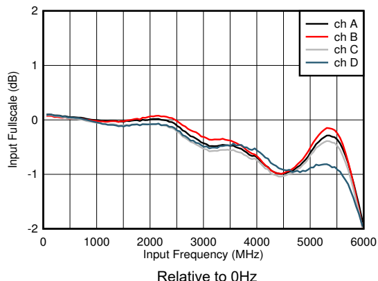
FIG 8-3. Input Fullscale vs Frequency
