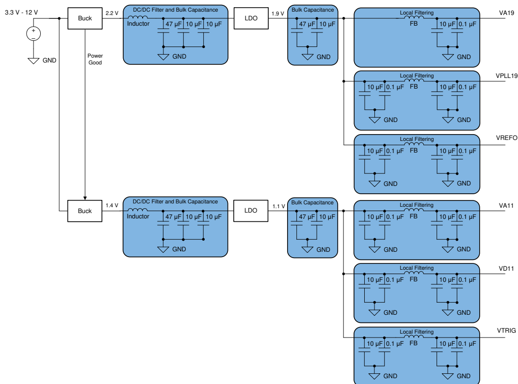
11-1. LDO Linear Regulator Approach Example
