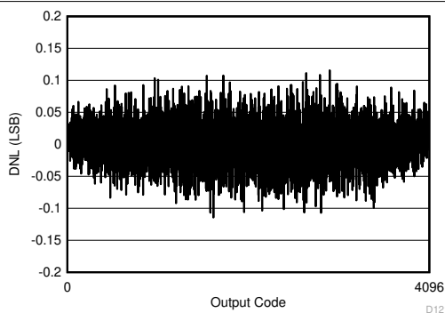
FIG 8-1. DNL vs Code
