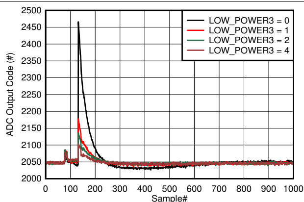
图 9-12. Background Calibration Core Transition In Low Power Mode
