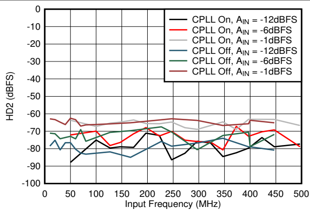
FIG 8-58. HD2 vs A_{IN} and C-PLL
