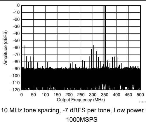
Figure 8-72. Two Tone FFT at 348 MHz
