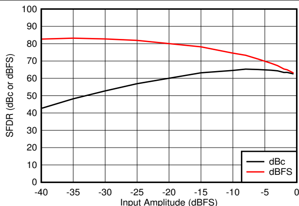
8-32. SFDR vs A_{IN}
