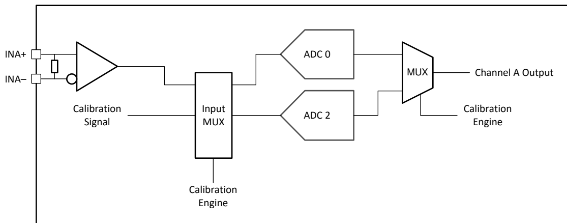
9-17. Single Channel Calibration System Block Diagram
