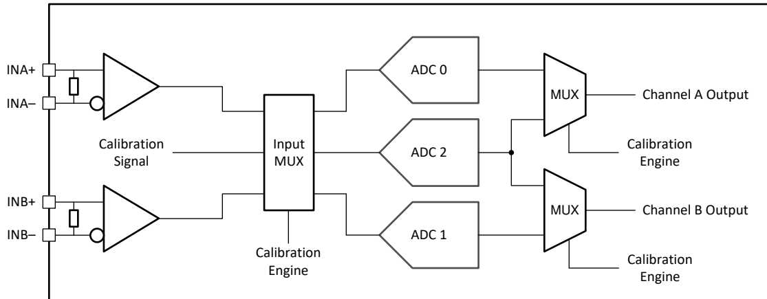
9-16. DualChannel Calibration System Block Diagram
