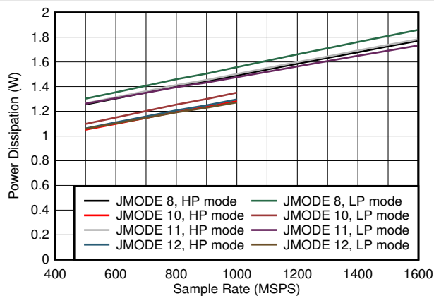
FIG 7-91. Dual Channel, Power Dissipation vs F_S and JMODE 8 - 12
