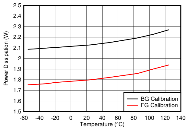
7-122. Dual Channel, Power Dissipation vs Temperature
