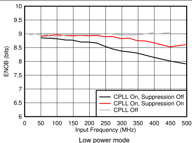
FIG 7-47. ENOB vs F_{IN} and C-PLL modes
