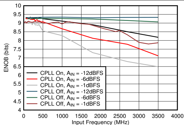
FIG 7-51. ENOB vs A_{IN} and C-PLL
