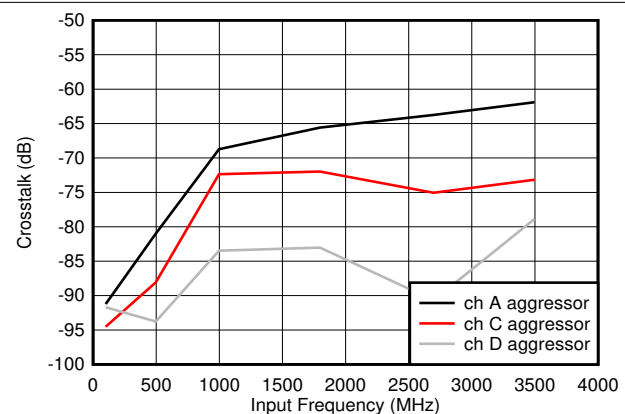
FIG 7-78. Crosstalk to Channel B vs F_{IN}
