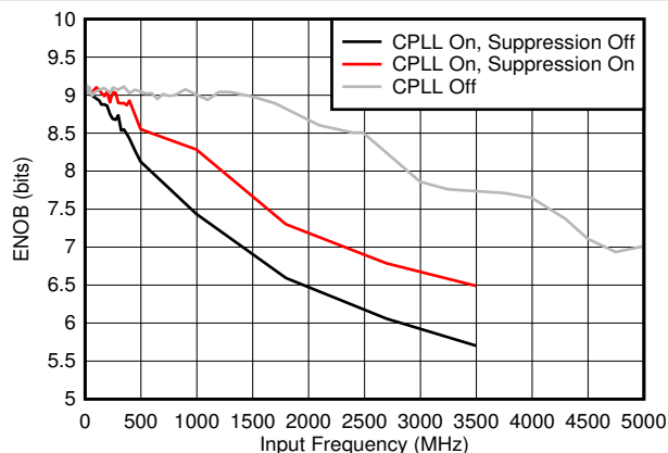
FIG 7-43. ENOB vs F_{IN} and C-PLL modes
