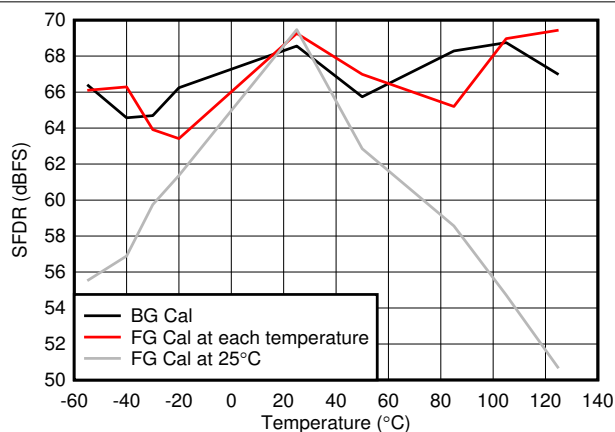
FIG 7-65. SFDR vs Temperature
