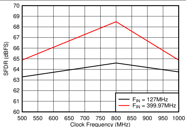
7-27. SFDR vs Sample Rate
