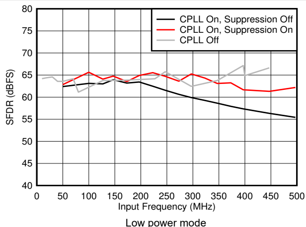
FIG 7-44. SFDR vs F_{IN} and C-PLL modes
