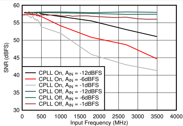
FIG 7-49. SNR vs A_{IN} and C-PLL
