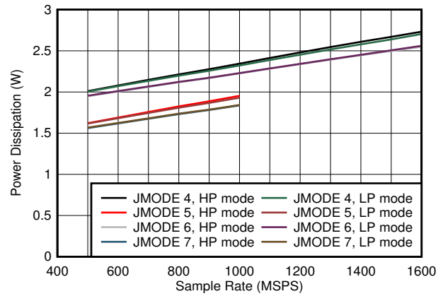
7-80. Quad Channel, Power Dissipation vs F_S and JMODE 4 - 7
