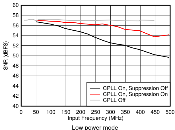
FIG 7-45. SNR vs F_{IN} and C-PLL modes
