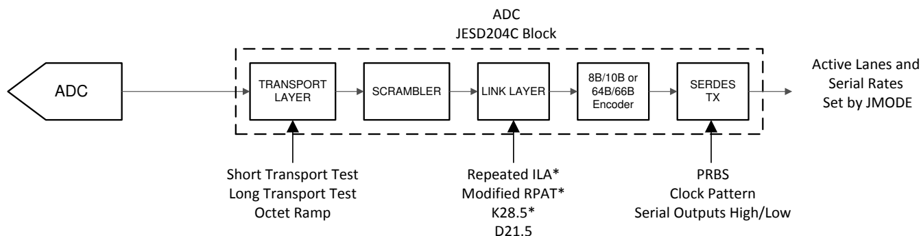
Figure 8-12. Test Mode Insertion Points
