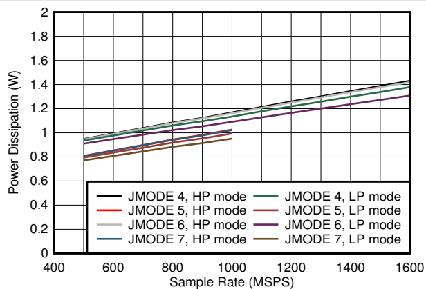
7-100. Single Channel, Power Dissipation vs F_S and JMODE 4 - 7
