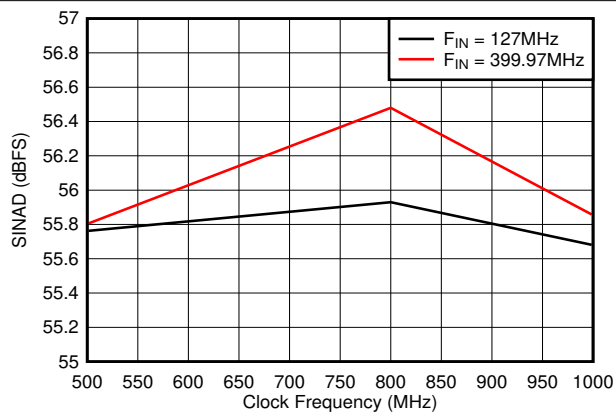
7-30. SINAD vs Sample Rate
