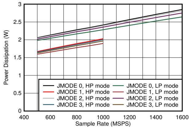
7-79. Quad Channel, Power Dissipation vs F_S and JMODES 0 - 3
