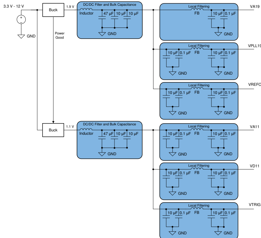
9-4. Switcher-Only Approach Example
