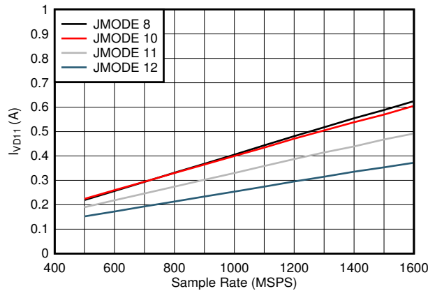
7-87. Quad Channel, I_{VD11} vs F_S and JMODE 8 - 12
