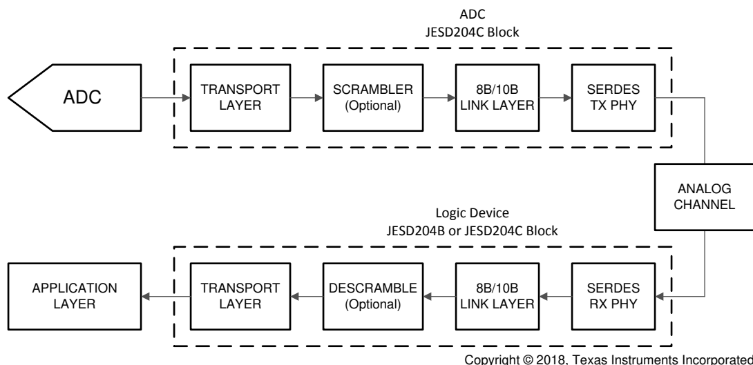
8-5. Simplified 8B/10B Encoded JESD204C Interface Diagram
