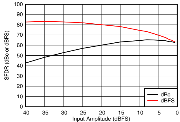
7-32. SFDR vs A_{IN}
