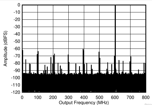
7-8. Single Tone FFT at 997 MHz and -1 dBFS
