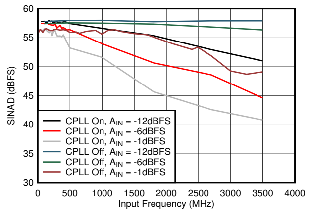
FIG 7-50. SINAD vs A_{IN} and C-PLL
