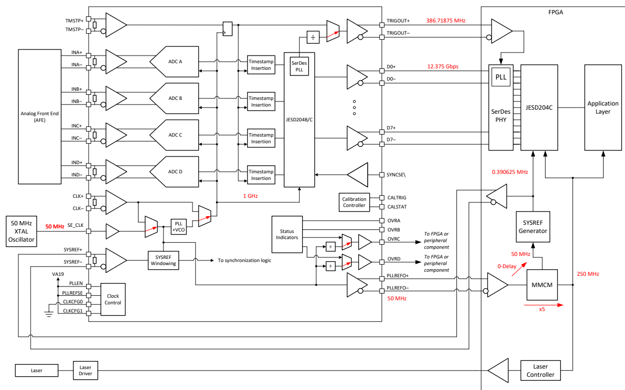
9-1. Typical Configuration for a LiDAR Digitizer
