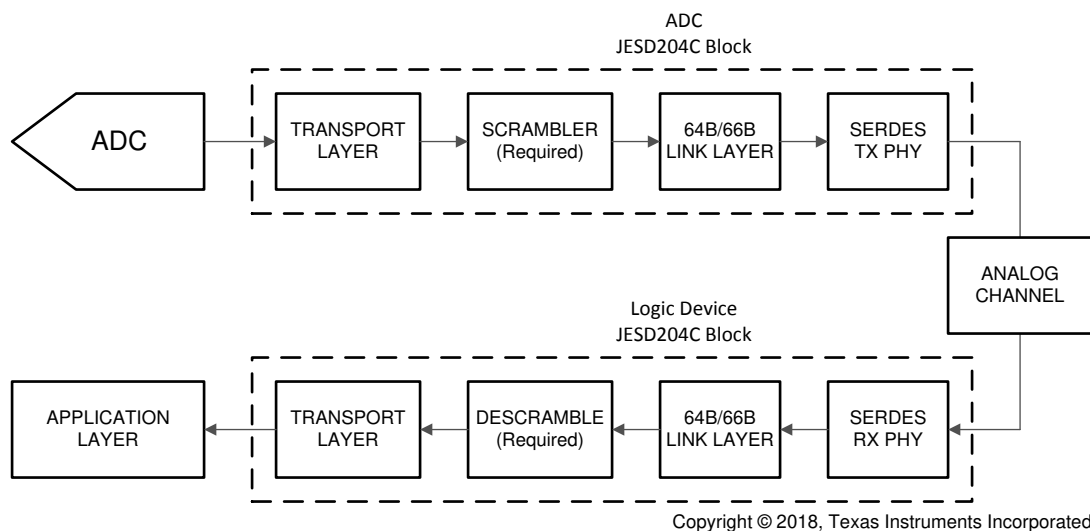
8-6. Simplified 64B/66B Encoded JESD204C Interface Diagram
