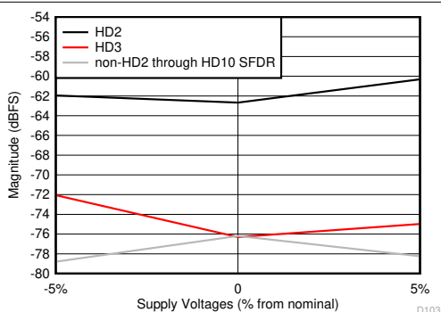
FIG 7-61. HD2, HD3 and Worst non-HD Spur vs Supply Voltage
