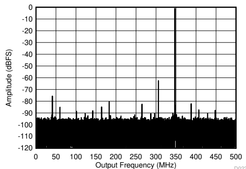
7-10. Single Tone FFT at 1797 MHz and -1 dBFS
