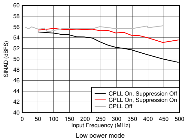
FIG 7-46. SINAD vs F_{IN} and C-PLL modes
