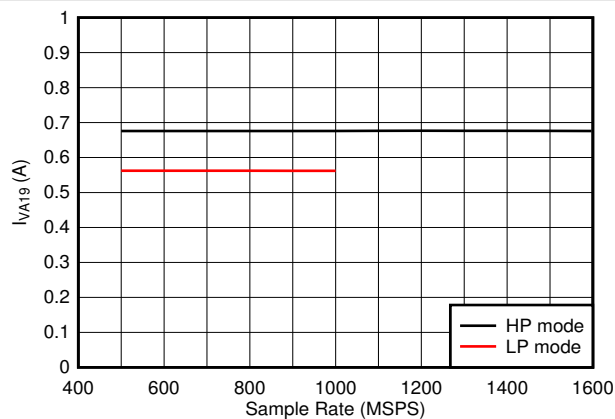
7-83. Quad Channel, I_{VA19} vs F_S
