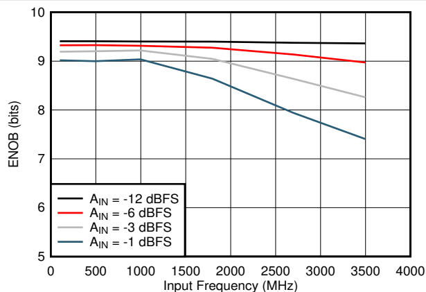
7-20. ENOB vs Input Frequency
