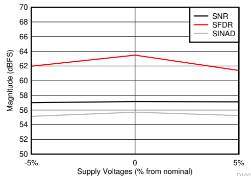
Figure 7-60. SNR, SFDR and SINAD vs Supply Voltage
