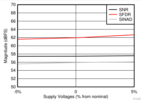
FIG 7-62. SNR, SFDR and SINAD vs Supply Voltages
