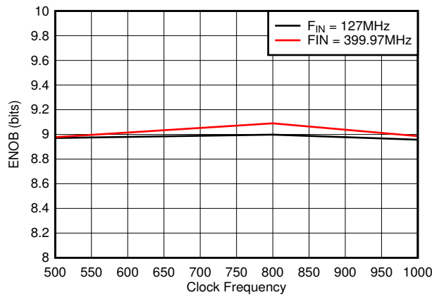
7-31. ENOB vs Sample Rate
