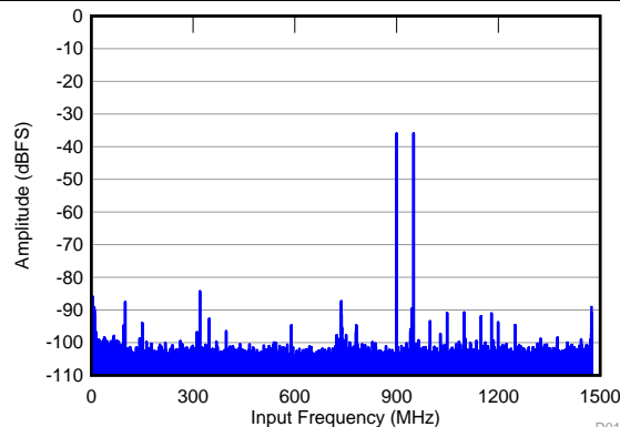
f_{IN1} = 900 \text{ MHz} , f_{IN2} = 950 \text{ MHz} , A_{IN} = -36 \text{ dBFS} , \text{IMD} = 94 \text{ dBFS}
