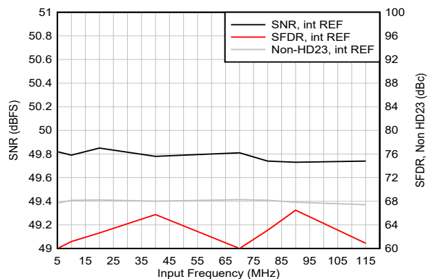
Figure 6-43. AC Performance vs Input Frequency
