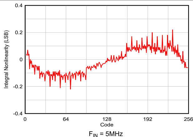
6-30. INL vs ADC Code
