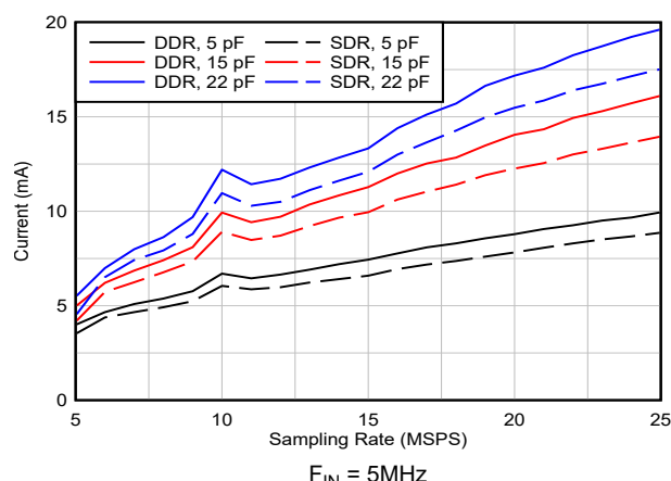
図 6-18. I_{IOVDD} Current vs Load Capacitance
