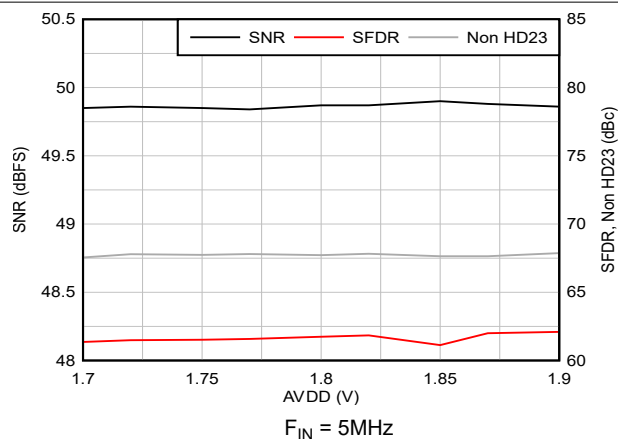
6-28. AC Performance vs AVDD
