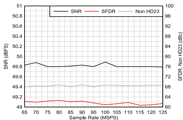
Figure 6-45. AC Performance vs Sampling Rate
