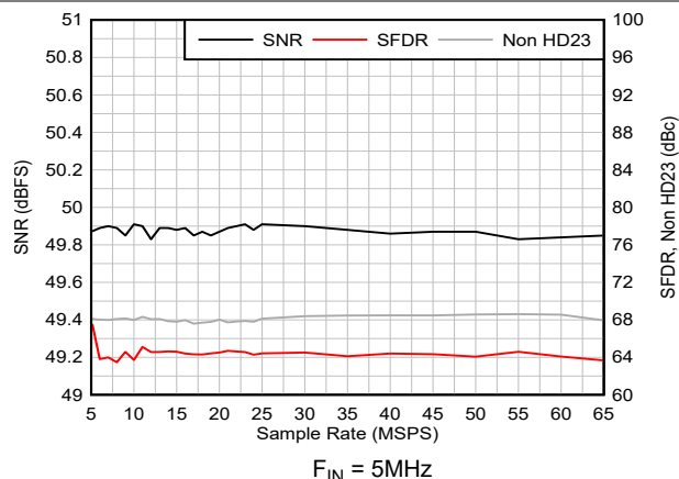
6-26. AC Performance vs Sampling Rate
