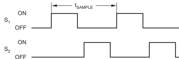
Figure 7-5. S_1 and S_2 Switch Timing
