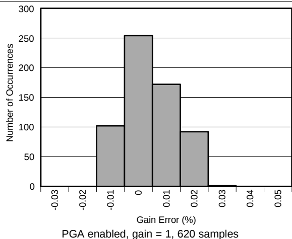
FIG 18. Gain Error Histogram
