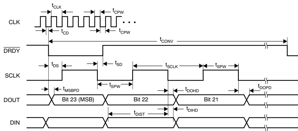
Figure 1. SPI Format Timing Characteristics
