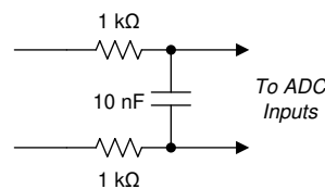
☒ 9-1. Recommended Antialiasing Circuitry
