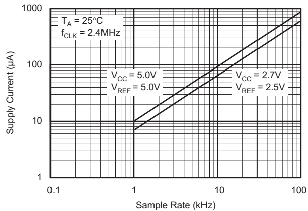
Figure 23. Maintaining f_{CLK} at the Highest Possible Rate Allows Supply Current to Drop Linearly With Sample Rate
