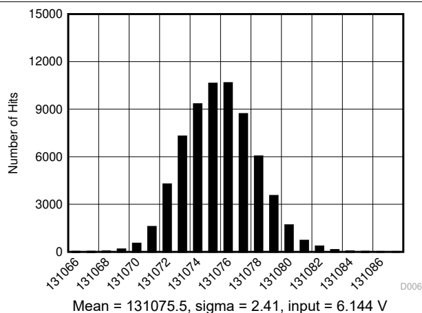
FIG 6-18. DC Histogram for Mid-Scale Inputs (0 V–12.288 V)
