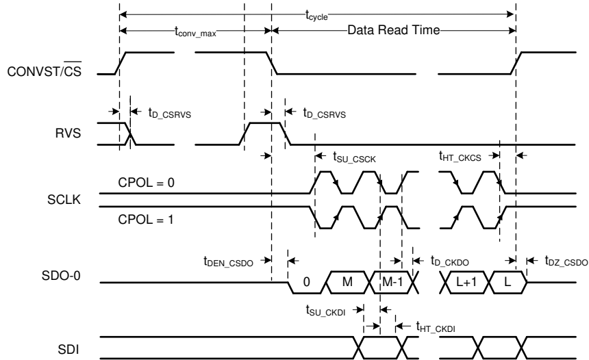
FIG 6-4. Standard SPI Interface Timing Diagram for CPHA = 1
