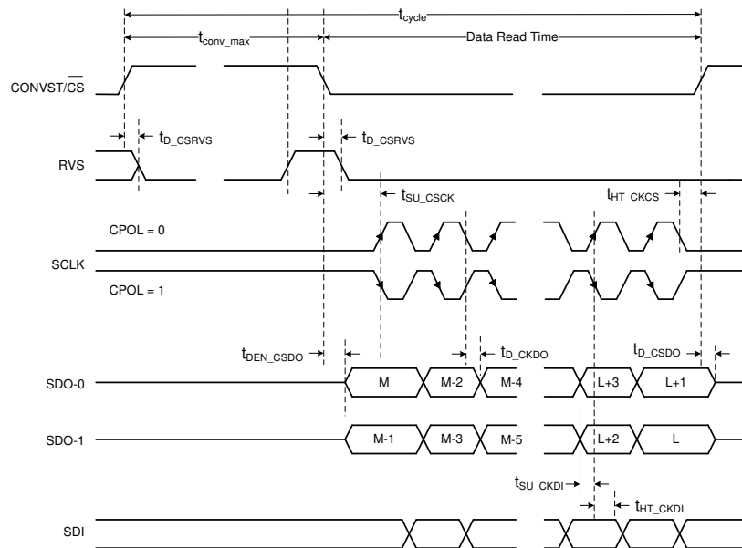
FIG 6-5. multiSPI Interface Timing Diagram for Dual SDO-x and CPHA = 0
