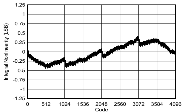
6-7. Integral Linearity Error vs Code
