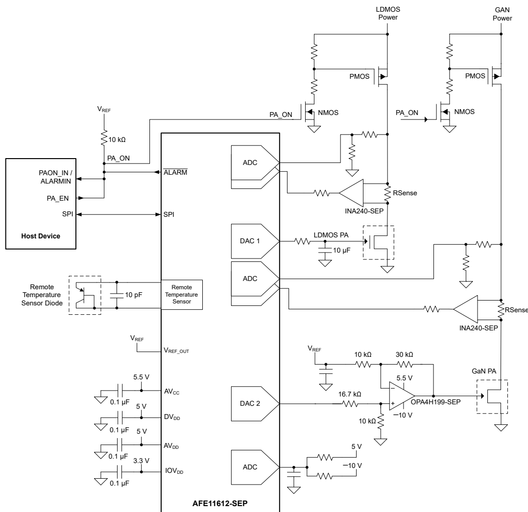
8-1. Power Amplifier (PA) Biasing
