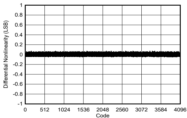
6-6. Differential Linearity Error vs Code
