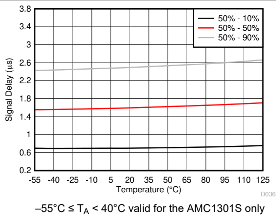
FIG 6-39. V_{IN} to V_{OUT} Signal Delay vs Temperature
