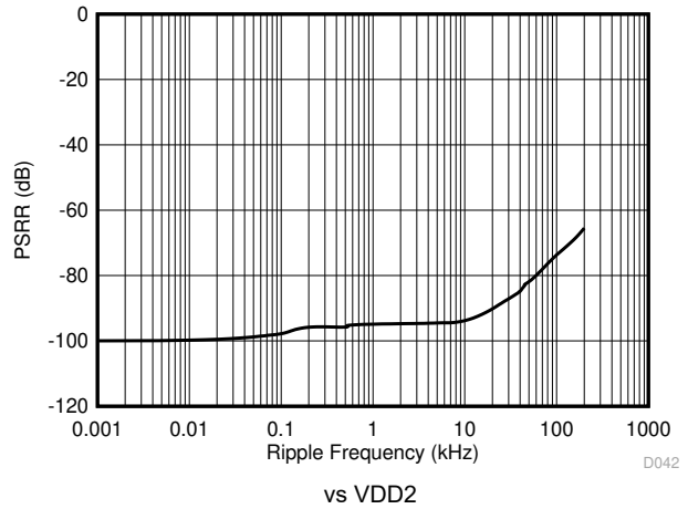
FIG 6-36. Power-Supply Rejection Ratio vs Ripple Frequency
