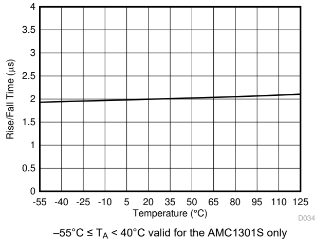
FIG 6-37. Output Rise and Fall Time vs Temperature
