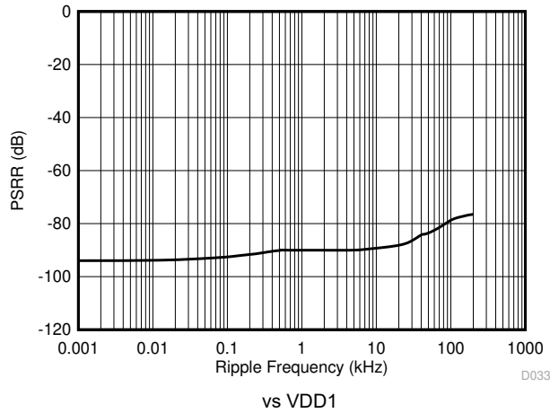
FIG 6-35. Power-Supply Rejection Ratio vs Ripple Frequency
