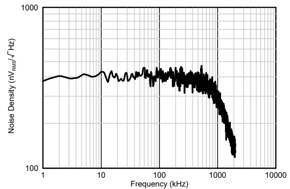
FIG 6-17. Noise Spectral Density vs Frequency
