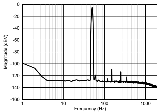
FIG 6-16. Frequency Spectrum With 50-Hz Input Signal
