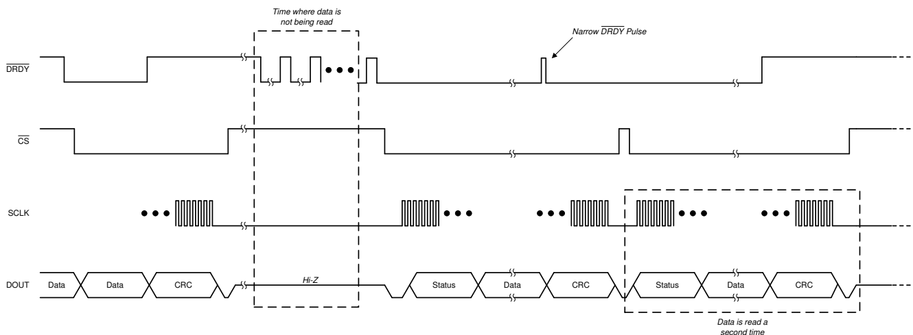
図 8-32. Collecting Data After a Pause by Reading Data Twice
