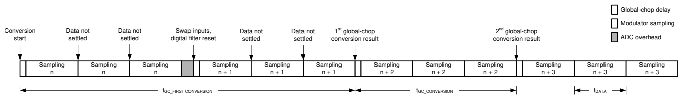
図 8-23. Conversion Timing With Global-Chop Mode Enabled
