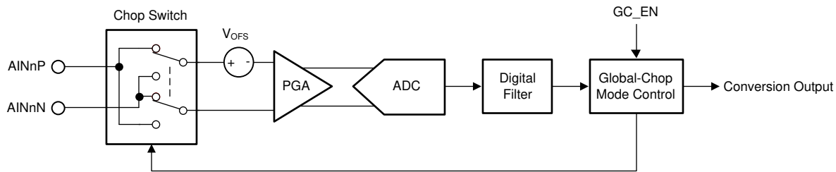
図 8-22. Global-Chop Mode Implementation
