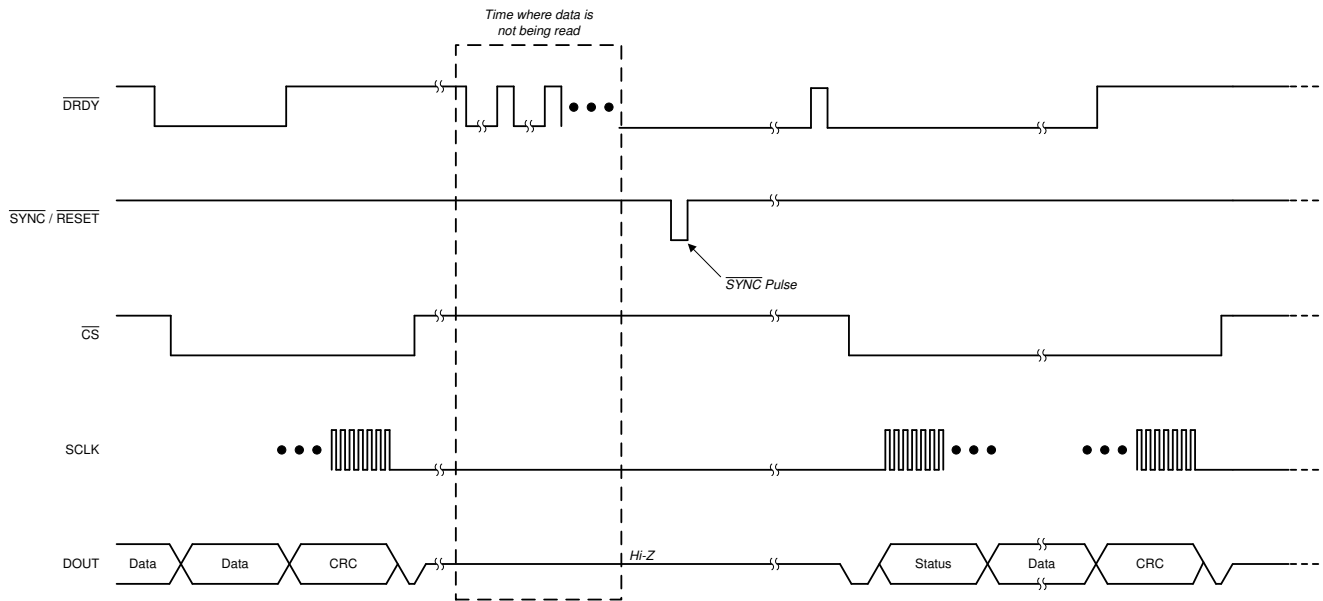
図 8-31. Collecting Data After a Pause Using the SYNC/RESET Pin
