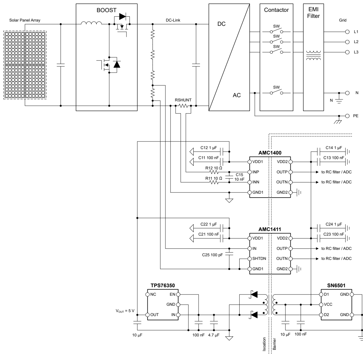
8-1. Using the AMC1400 for Current Sensing in a Typical Application
