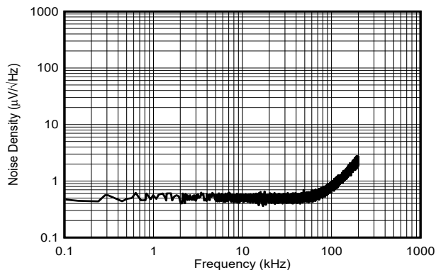
6-24. Input-Referred Noise Density vs Frequency
