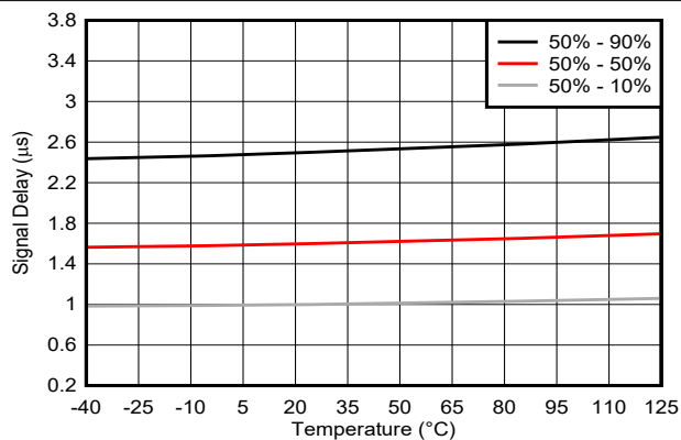
FIG 6-35. IN to OUTP, OUTN Signal Delay vs Temperature
