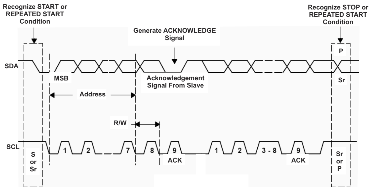
図 8-13. BUS Protocol
