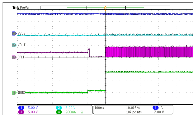
図 9-3. Switched Cap Mode Power Up
