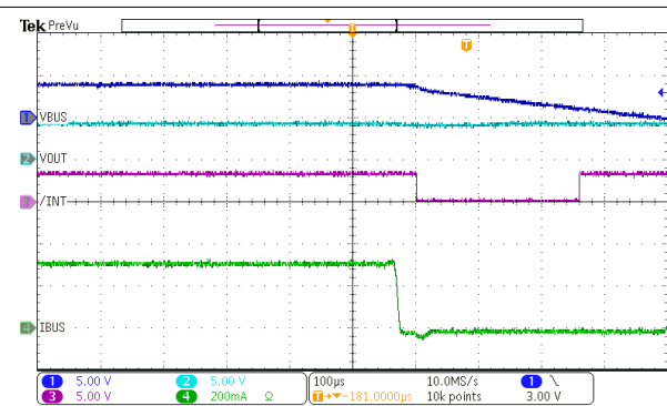
図 9-6. Adapter Unplug in Bypass Mode
