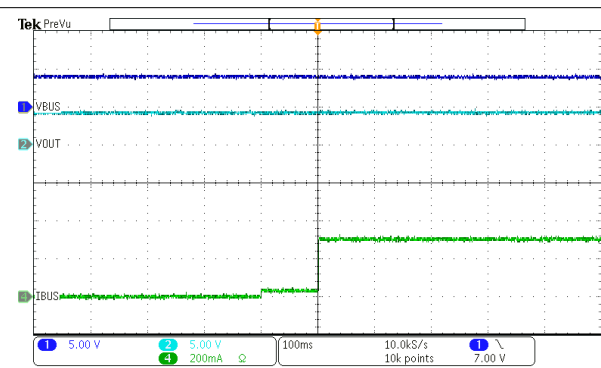
図 9-4. Bypass Mode Power Up
