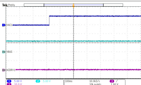
図 9-16. Power Up from VAC1 with Single ACFET1
