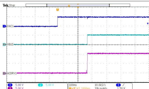
図 9-15. Power Up without AC-RFFET
