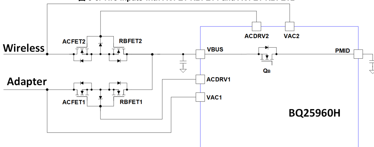
図 8-6. Two Inputs with ACFET-RBFET1 and ACFET-RBFET2
