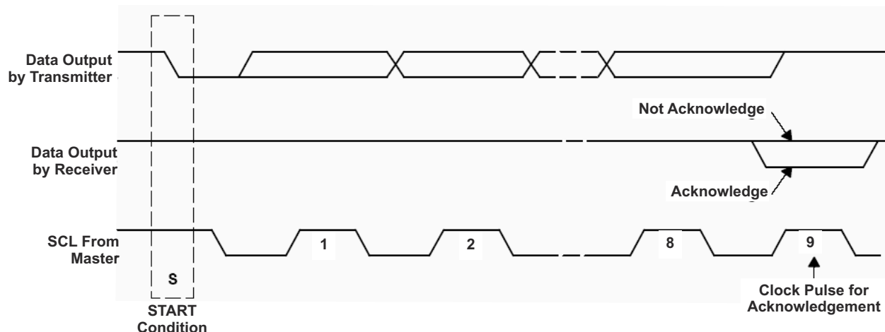
図 8-12. Acknowledge on the I 2 C BUS
