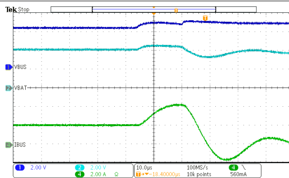
図 9-8. VBUSOVP in Bypass Mode
