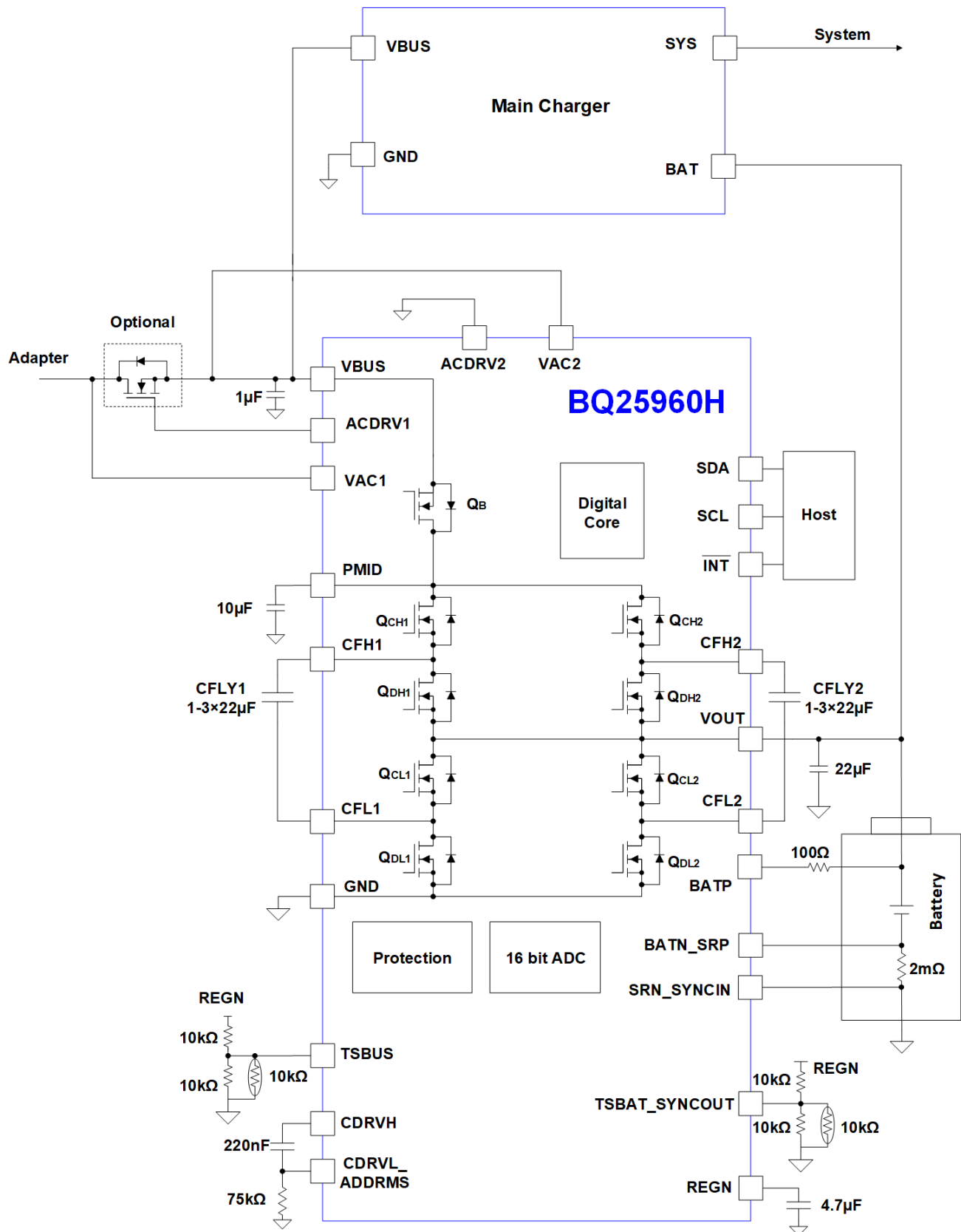
9-2. BQ25960H Typical Application Diagram with Single Input
