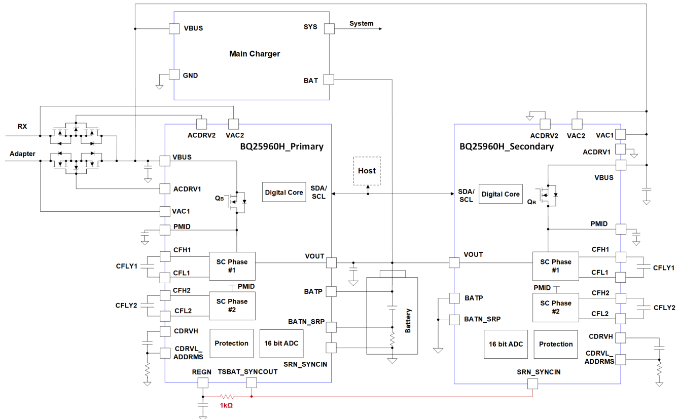
図 8-9. Parallel Operation of BQ25960H
