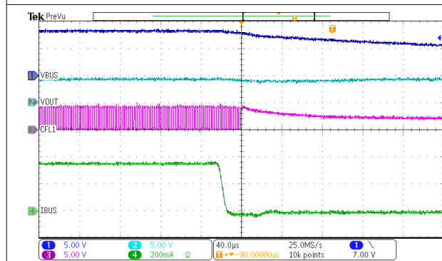
図 9-5. Adapter Unplug in Switched Cap Mode
