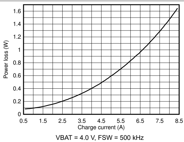
7-6. Battery Charge Power Loss vs. Charge Current, 3 x 22- \mu F CFLY per Phase
