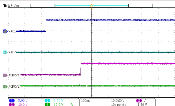
図 9-17. Power Up from VAC1 with ACFET1-RBFET1
