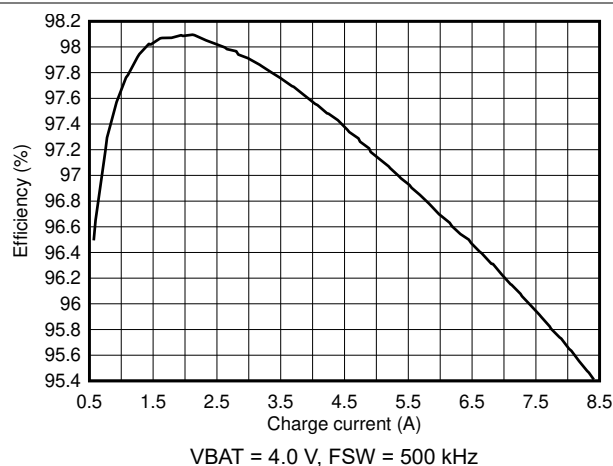
7-5. Battery Charge Efficiency vs. Charge Current, 3 x 22- \mu F CFLY per Phase
