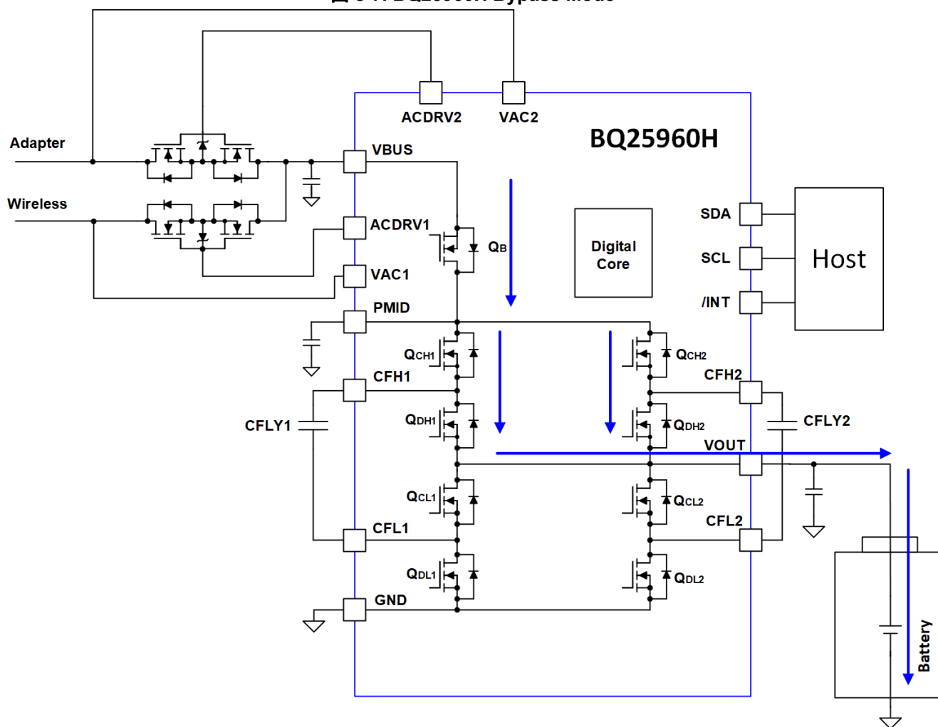
8-7. BQ25960H Bypass Mode
