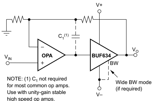
8-6. Boosting Op Amp Output Current
