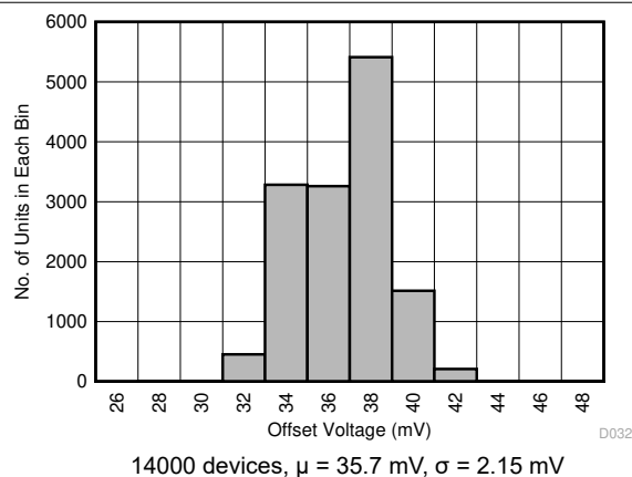
図 6-42. Offset Voltage Distribution Histogram
