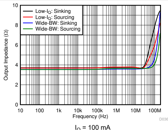
図 6-40. Output Impedance vs Frequency
