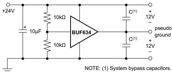
8-3. Pseudo-Ground Driver
