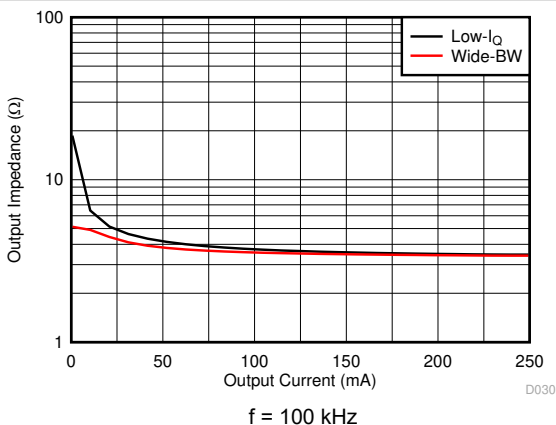
図 6-39. Output Impedance vs Output Current
