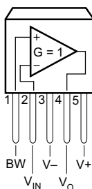
図 5-3. KTT Package, 5-Pin TO-263 (Top View)
