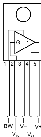
図 5-2. KC Package, 5-Pin TO-220 (Top View)
