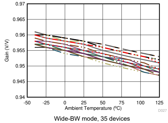
図 6-52. Buffer Gain vs Temperature
