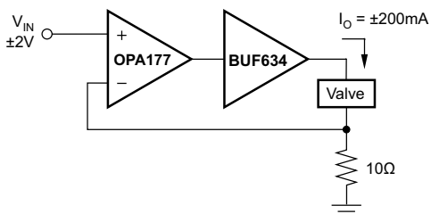
8-4. Current-Output Valve Driver
