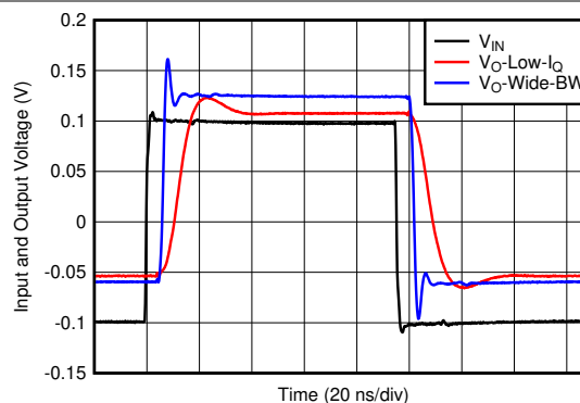
図 6-38. Small-Signal Transient Response
