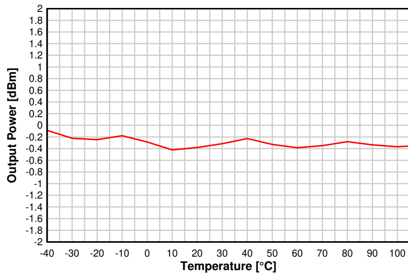
8-34. Output Power vs. Temperature (BLE 1 Mbps, 2.44 GHz)
