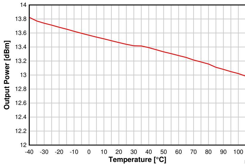
8-33. Output Power vs. Temperature (50 kbps, 868.3 MHz)
