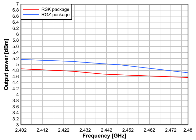
7-34. Output Power vs. Frequency (BLE 1Mbps, 2.44GHz, +5dBm)
