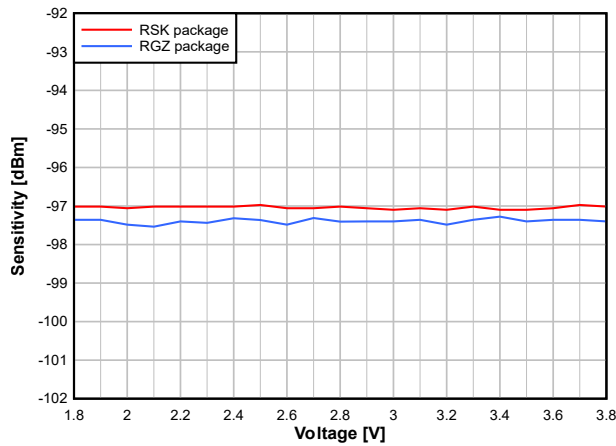
7-22. Sensitivity vs. Supply Voltage (VDD5) (BLE 1Mbps, 2.44GHz)
