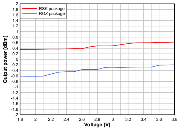
7-29. Output Power vs. Supply Voltage (VDDS) (BLE 1Mbps, 2.44GHz, 0dBm)
