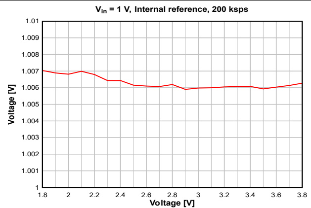
Figure 7-40. ADC Accuracy vs. Supply Voltage (VDD)
