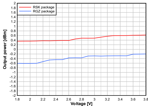
☒ 7-29. Output Power vs. Supply Voltage (VDDS) (BLE 1Mbps, 2.44GHz, 0dBm)
