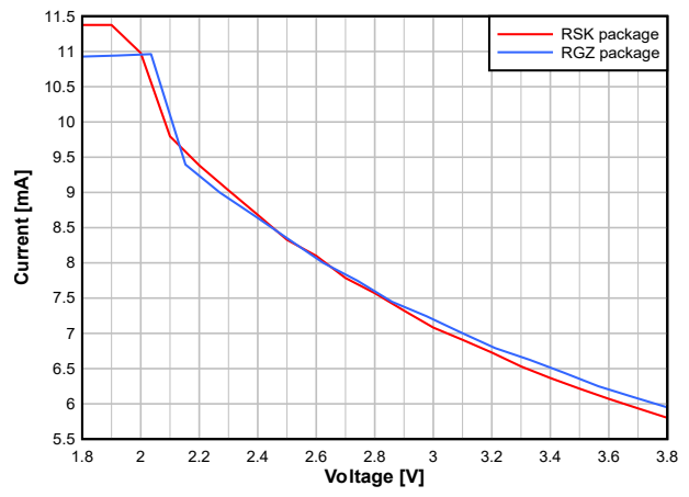
7-13. TX Current vs. Supply Voltage (VDDS) (BLE 1 Mbps, 2.44GHz, 0dBm)
