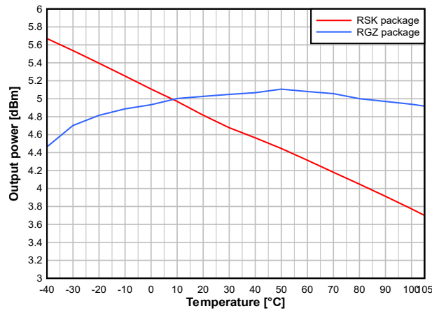
☒ 7-27. Output Power vs. Temperature (BLE 1Mbps, 2.44GHz, +5dBm)
