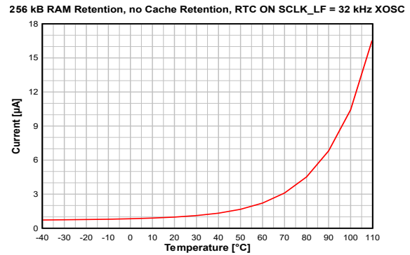
7-4. Standby Mode (MCU) Current vs. Temperature
