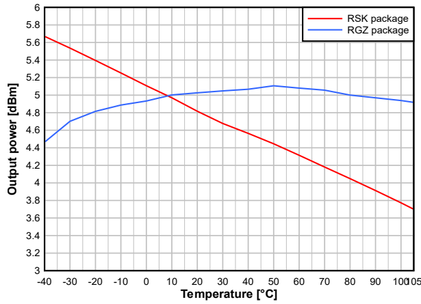
7-27. Output Power vs. Temperature (BLE 1Mbps, 2.44GHz, +5dBm)
