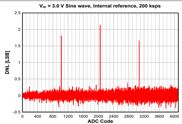
7-38. DNL vs. ADC Code
