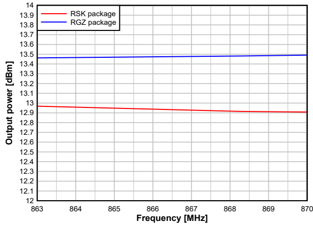
7-31. Output Power vs. Frequency (50kbps, 868MHz, +14dBm)
