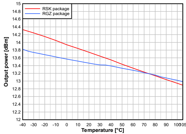
☒ 7-25. Output Power vs. Temperature (50kbps, 868.3MHz, +14dBm)
