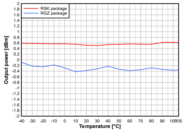
☒ 7-26. Output Power vs. Temperature (BLE 1Mbps, 2.44GHz, 0dBm)
