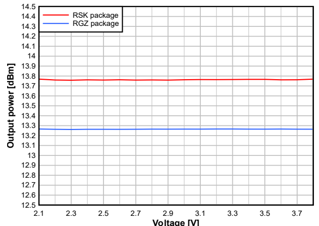
☒ 7-28. Output Power vs. Supply Voltage (VDDS) (50kbps, 868.3MHz, +14dBm)
