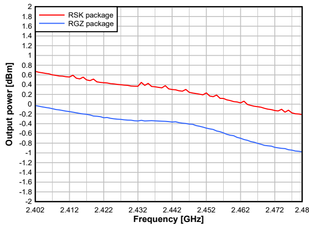
7-33. Output Power vs. Frequency (BLE 1Mbps, 2.44GHz, 0dBm)
