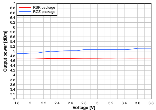
☒ 7-30. Output Power vs. Supply Voltage (VDDS) (BLE 1Mbps, 2.44GHz, +5dBm)
