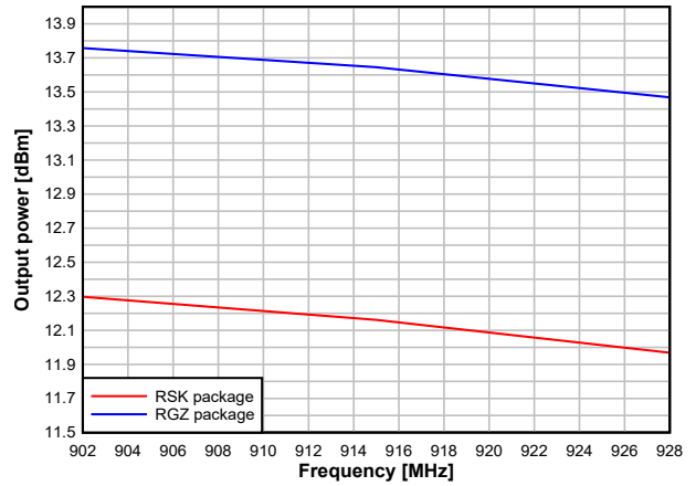
7-32. Output Power vs. Frequency (50kbps, 915MHz, +14dBm)
