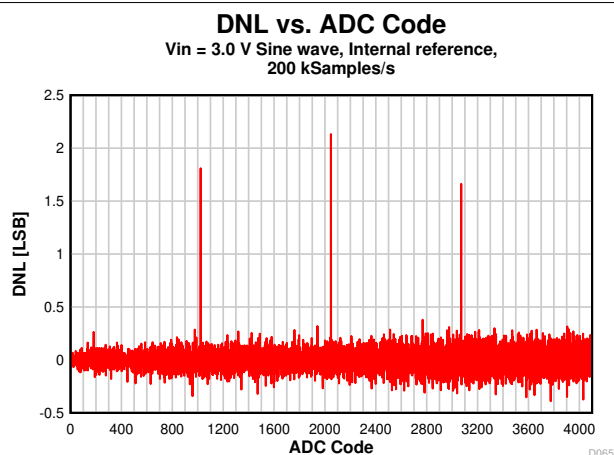
7-26. DNL vs. ADC Code
