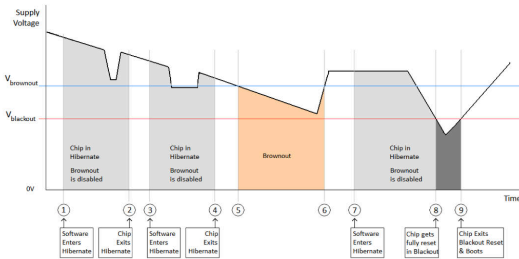
7-4. Brownout and Blackout Levels (1 of 2)
