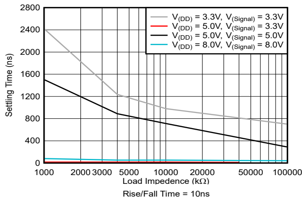
5-3. System Settling Time vs Signal Voltage
