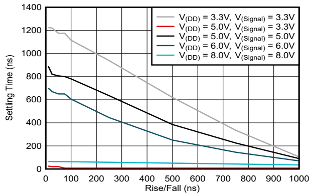
5-1. System Settling Time vs Signal Rise/Fall Time
