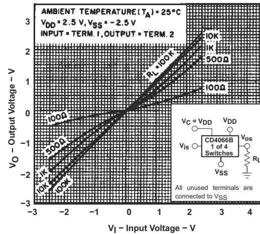
5-4. Typical ON Characteristics for 1 of 4 Channels
