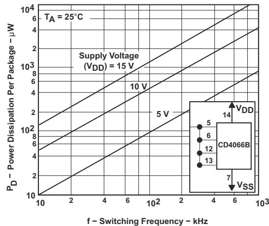
5-5. Power Dissipation per Package vs Switching Frequency
