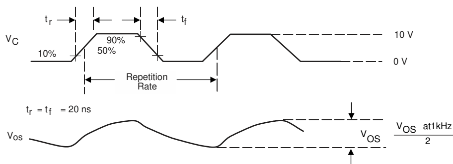
Figure 6-7. Propagation Delay, t_{PLH} , t_{PHL} Control-Signal Output
