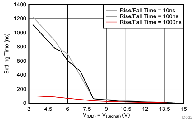
5-2. System Settling Time vs Signal Voltage
