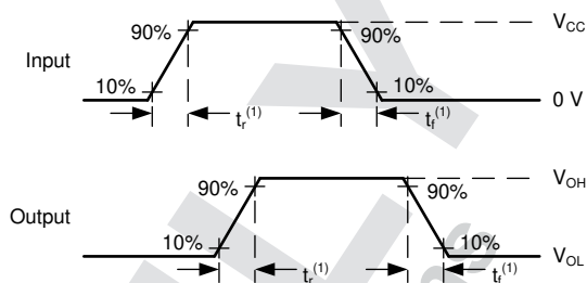
FIG 7-2. Voltage Waveforms Transition Times
