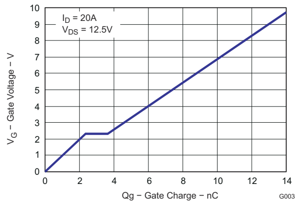
FIG 7-4. Gate Charge
