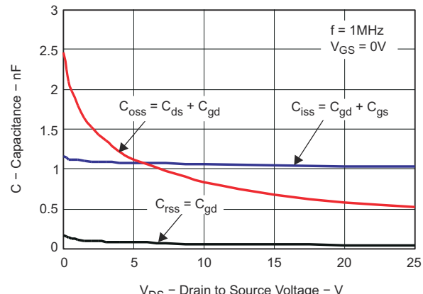
FIG 7-5. Capacitance
