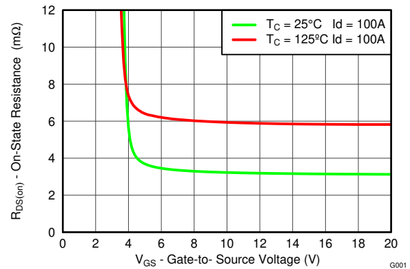
3-7. On-State Resistance vs Gate-to-Source Voltage
