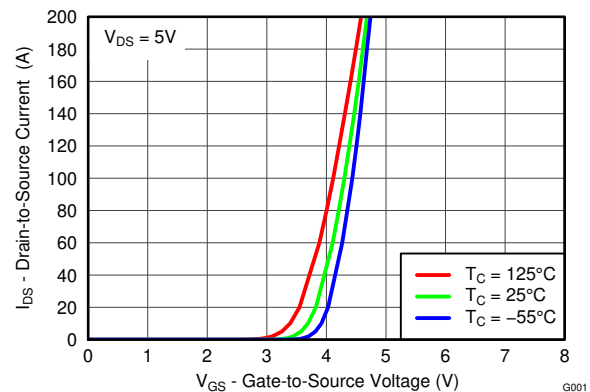
図 4-3. Transfer Characteristics
