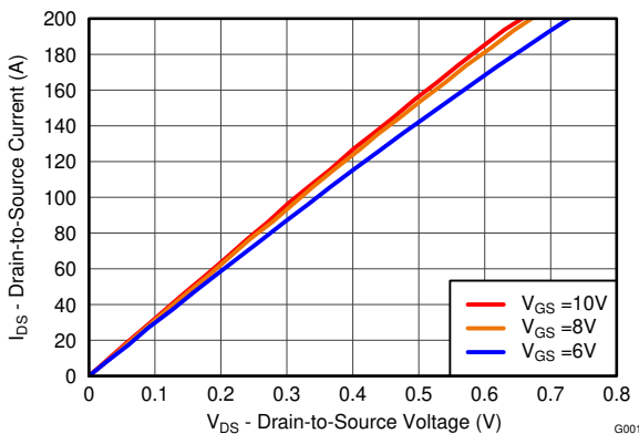
図 4-2. Saturation Characteristics
